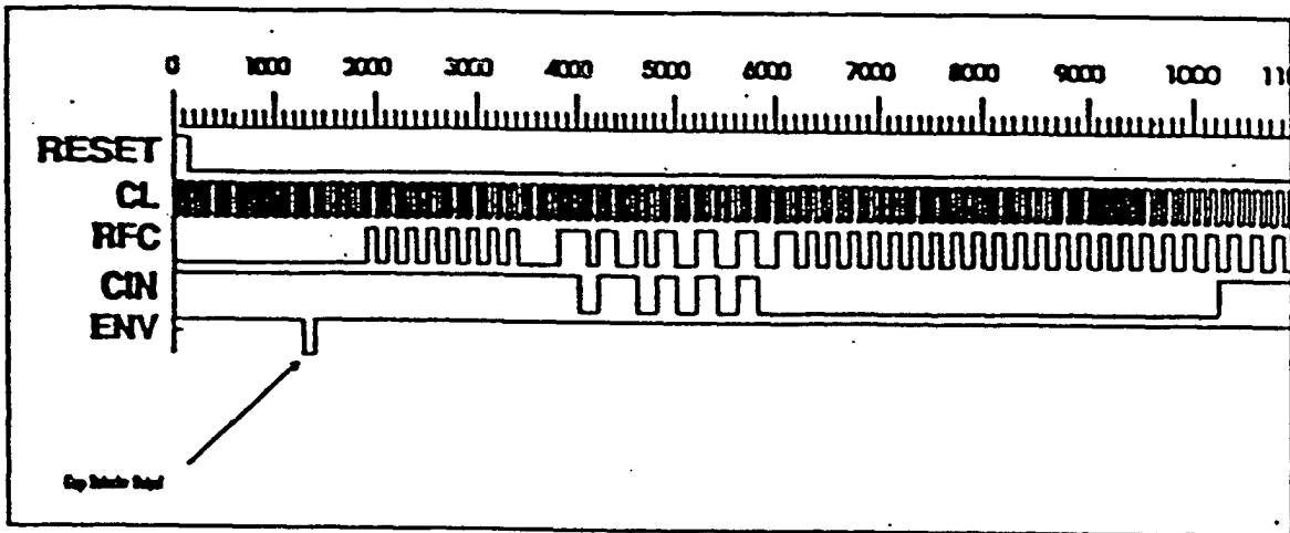
Waveforms with gap detection and synchronization
