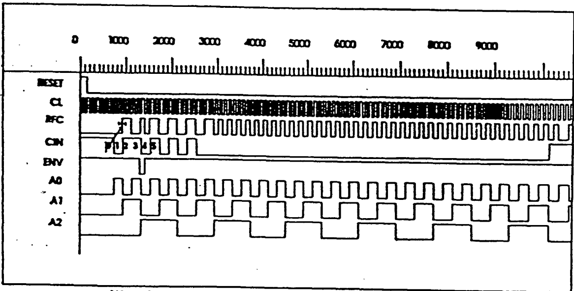
Waveforms with no gap detection or synchronization
