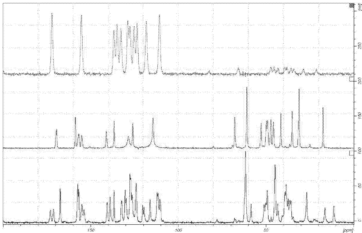
Figure F: Stacked plot of 13 C ss NMR spectra
