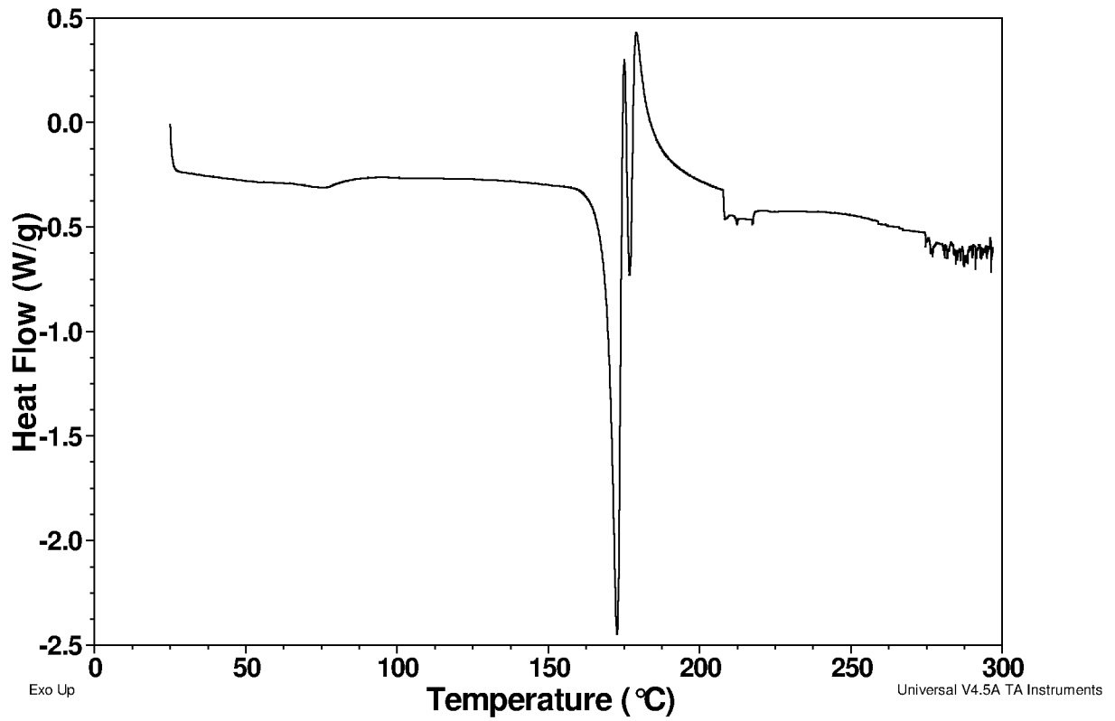
Figure L: DSC Thermogram of Compound A: 6-hydroxy-2-napthoic acid (1:1) co-crystal, Form B
