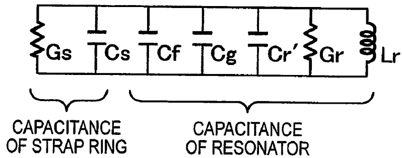
FIG. 8 (b) PRIOR ART
