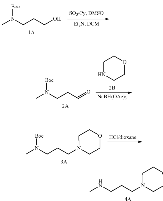
Scheme 4. Synthesis of N-methyl-3-morpholinopropan-1-amine (intermediate compound 4A).
