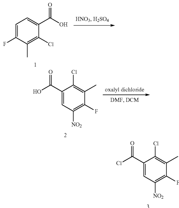
Scheme 1. Synthesis of 2-chloro-4-fluoro-3-methyl-5-nitrobenzoyl chloride (intermediate 3).
