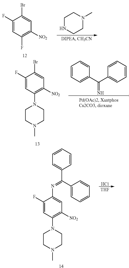
Scheme 5. Synthesis of methyl 1-(5-amino-2-fluoro-4-(4-methylpiperazin-1-yl)phenyl)-1H-1,2,3-triazole-4-carboxylate (common intermediate 18).
