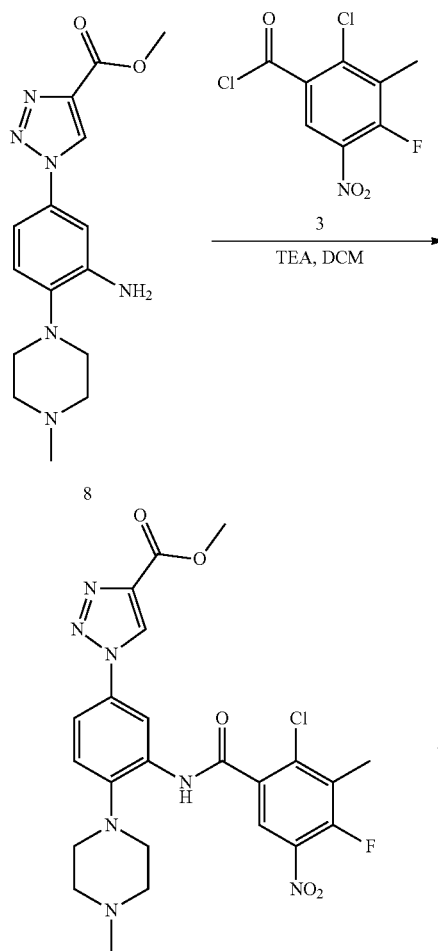
Scheme 2. Synthesis of 1-(3-(5-amino-2-chloro-4-fluoro-3-methylbenzamido)-4-(4-methylpiperazin-1-yl)phenyl)-1H-1,2,3-triazole-4-carboxylic acid (advanced intermediate 11) and Compound 2.
