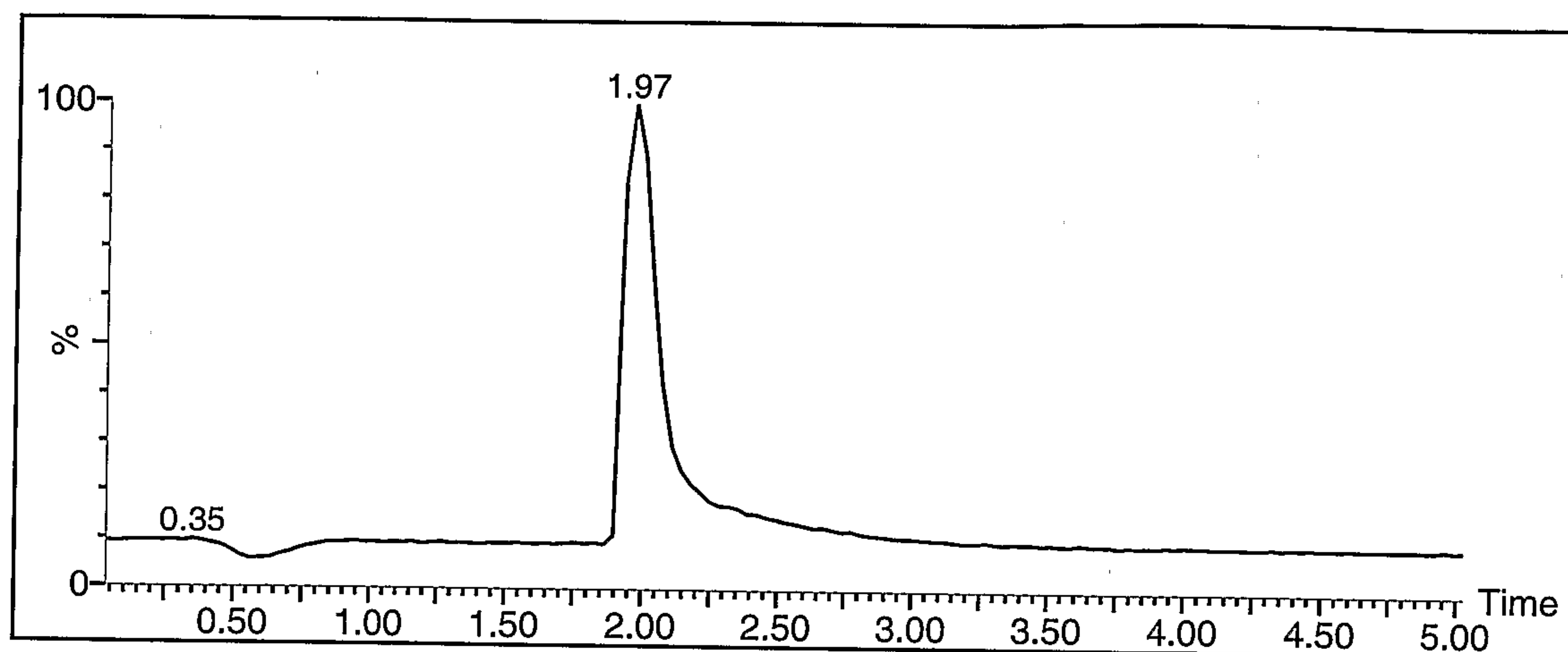
LC Trace - bis-MOM-dehydroequol
