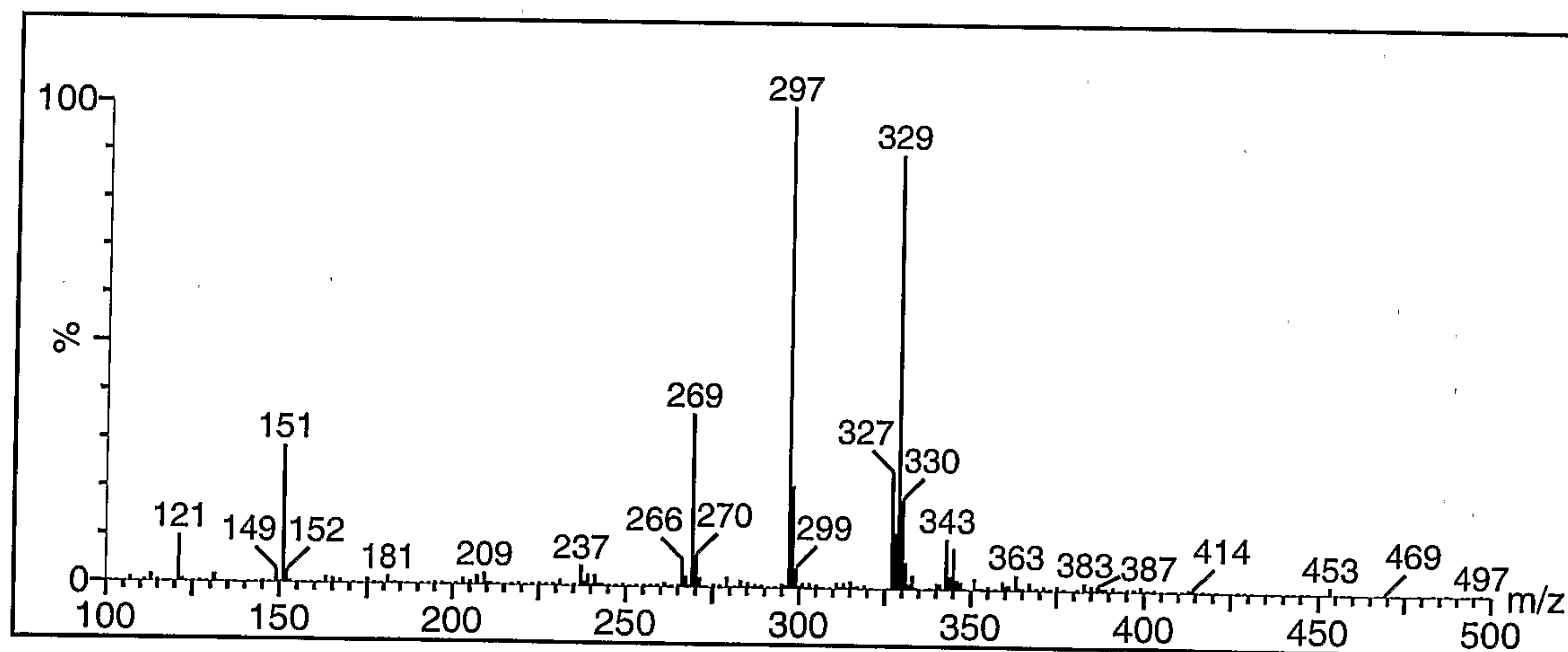
Spectrum - bis-MOM-dehydroequol
