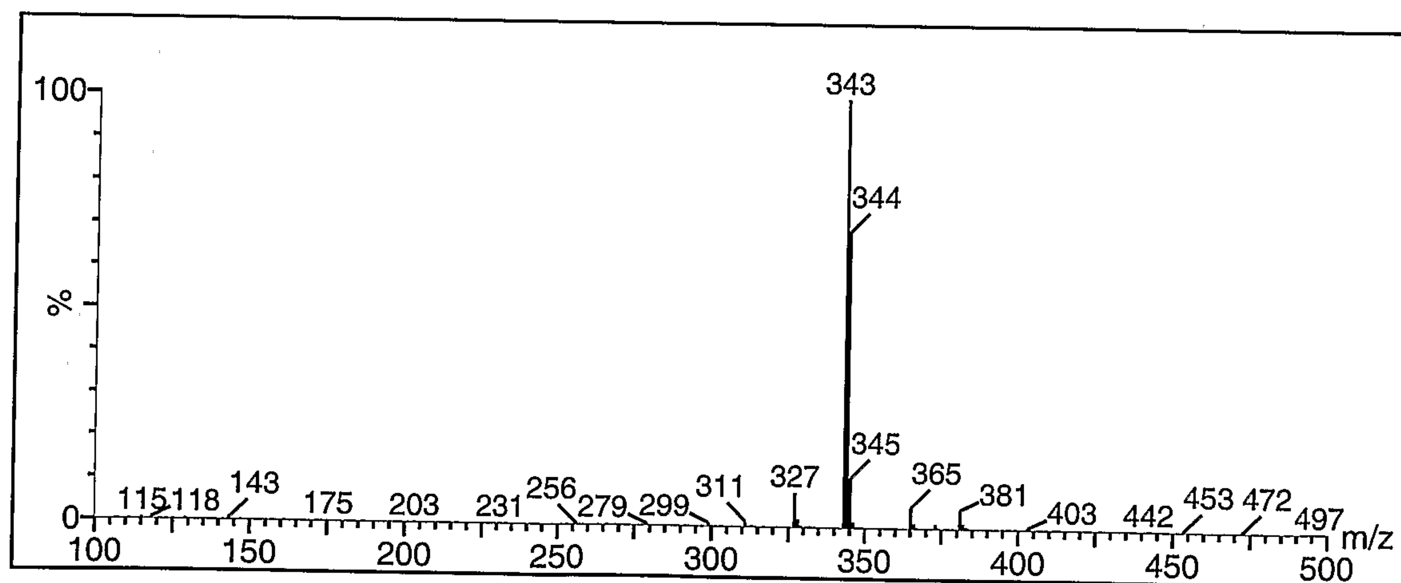
Spectrum - bis-MOM Daidzein
