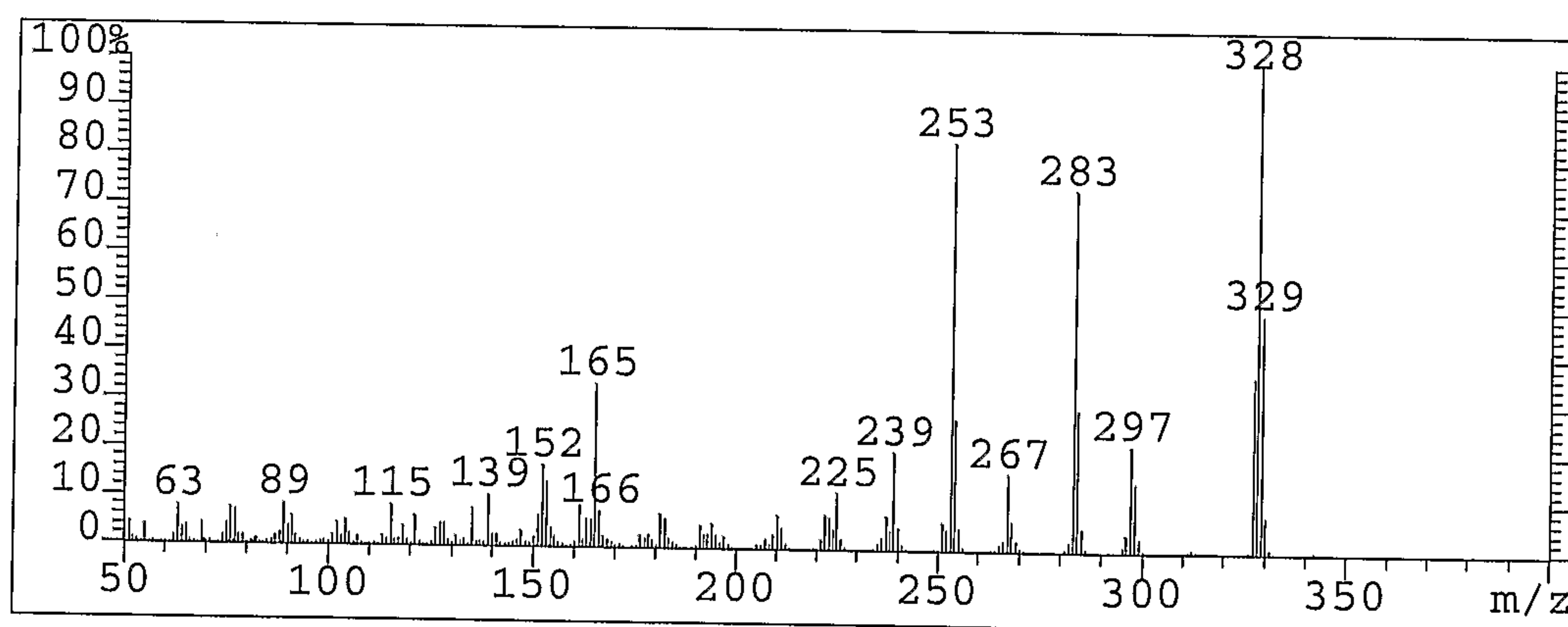
Spectrum - bis-MOM-dehydroequol
