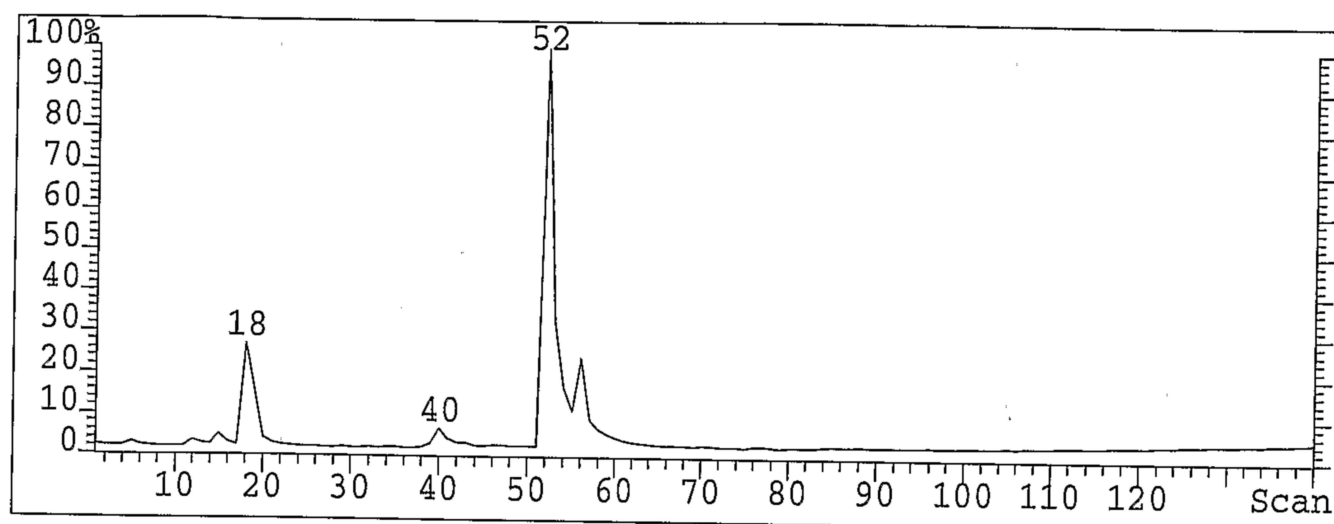
GC Trace - chroman-4-one
