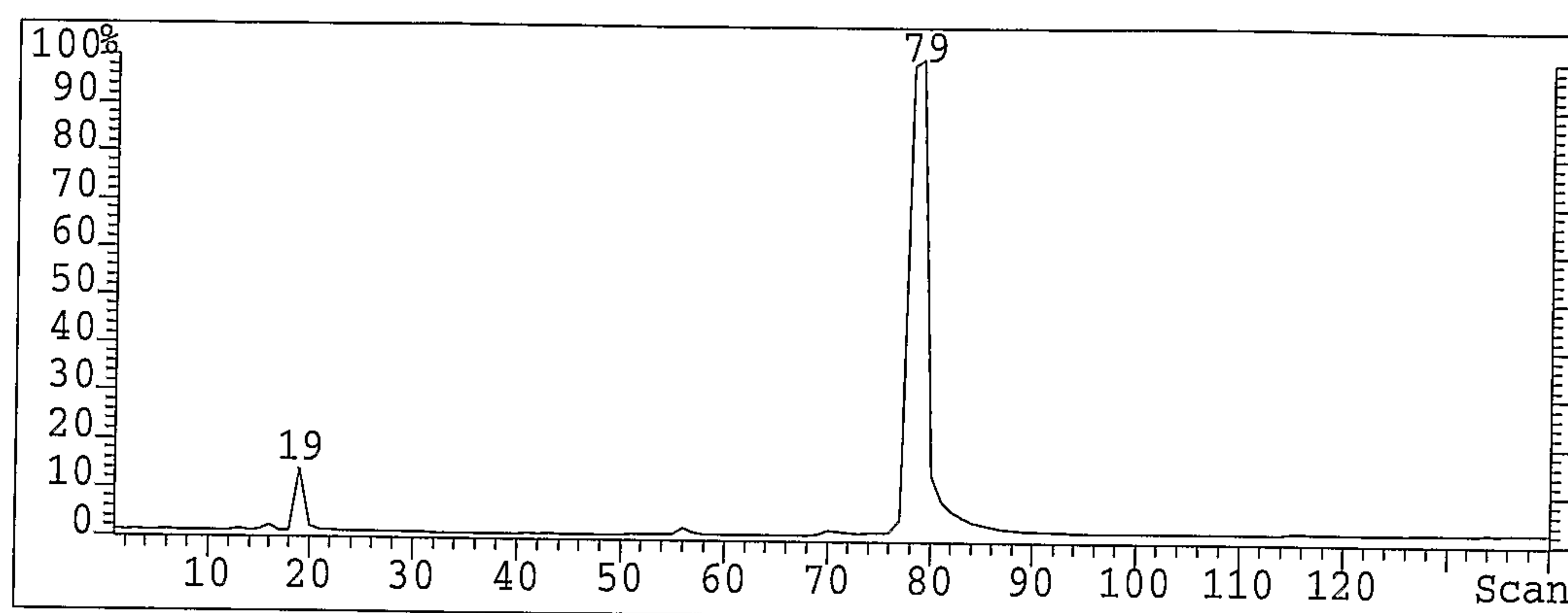
GC Trace - bis-MOM Daidzein
