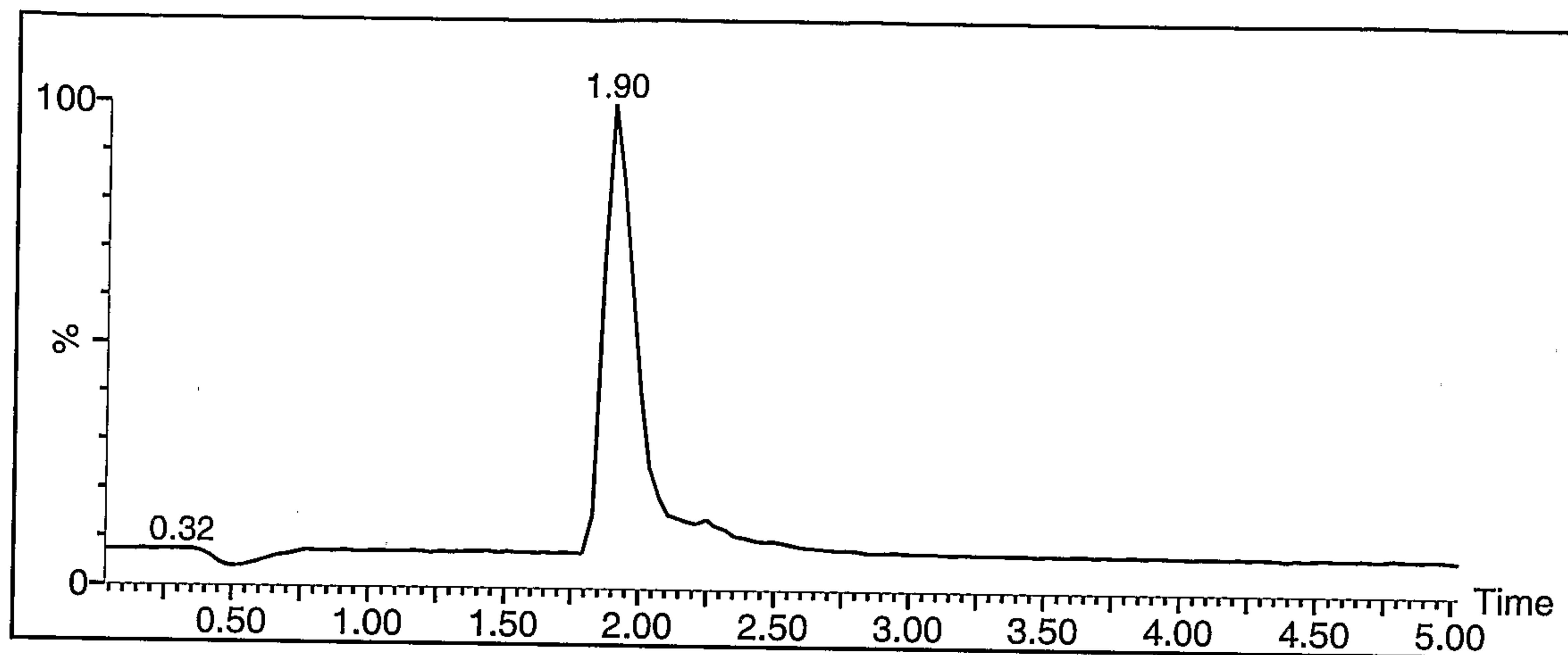
LC Trace - bis-MOM Daidzein
