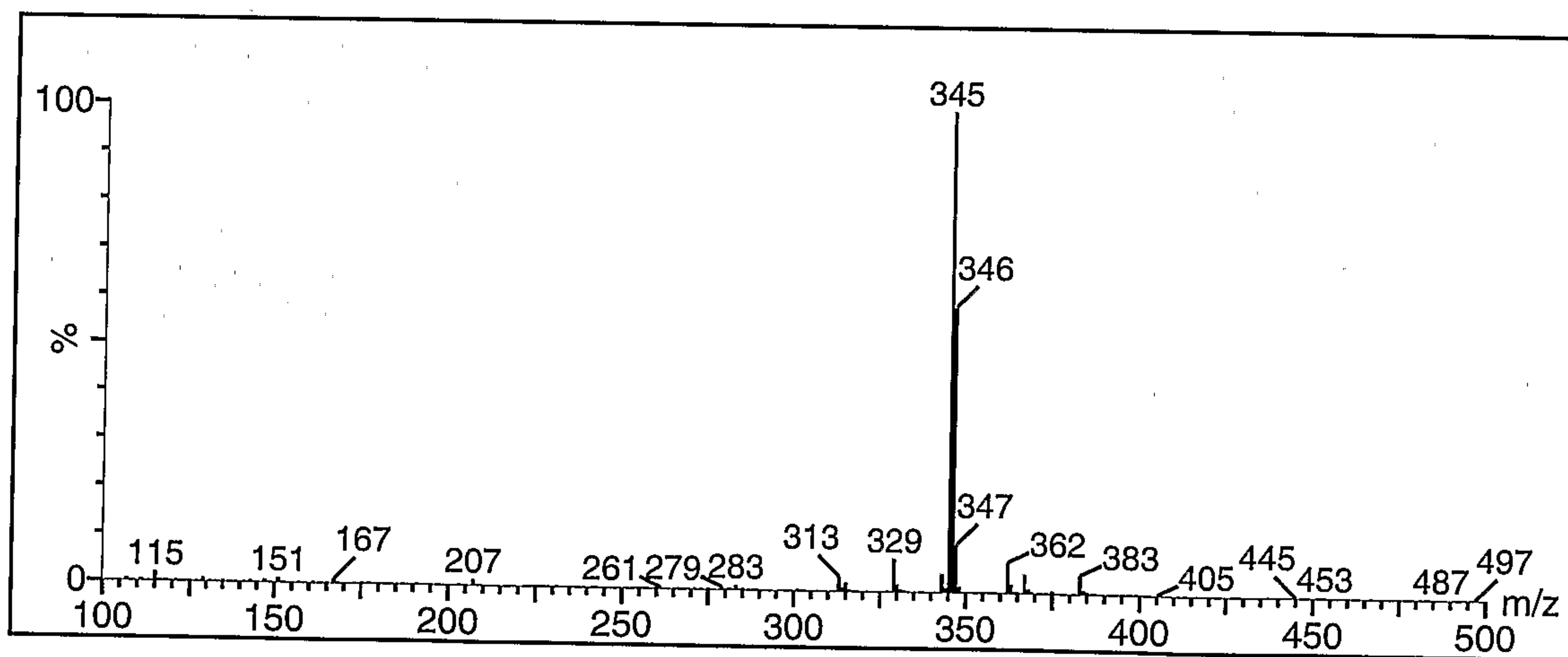
Spectrum - chroman-4-one
