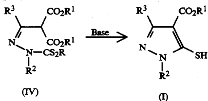
Reaction Scheme (2):
