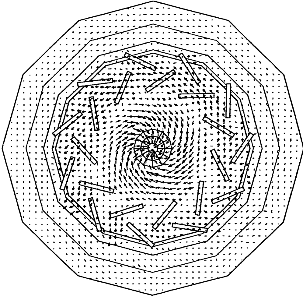
FIG. 4B ELECTRIC FIELD RIGHT BELOW MICROWAVE INTRODUCING WINDOW
