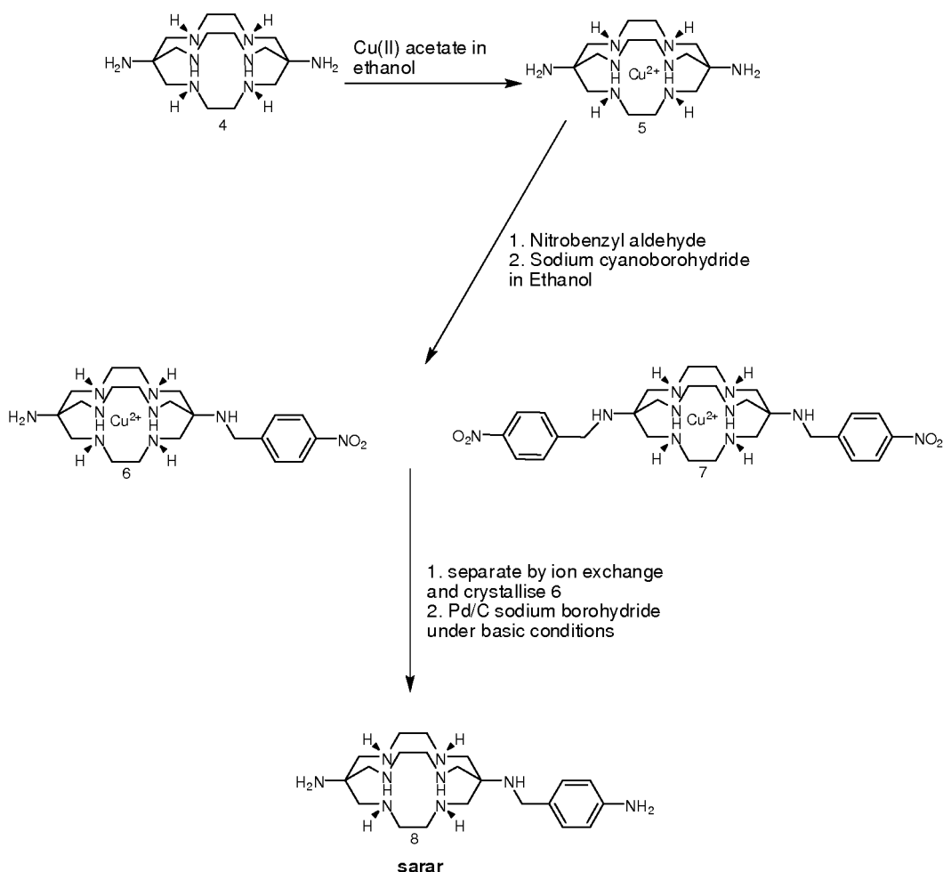
Scheme 2 – Synthesis of sarar (compound 8)
