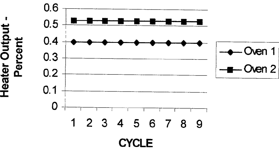
FIG 19 Chart 6: Twin Sheet Constant Heater Output
