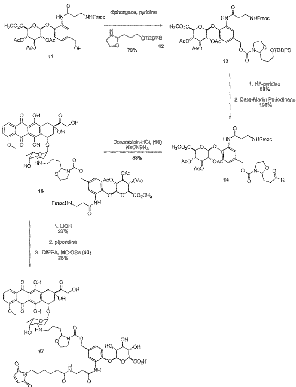
Scheme 4
