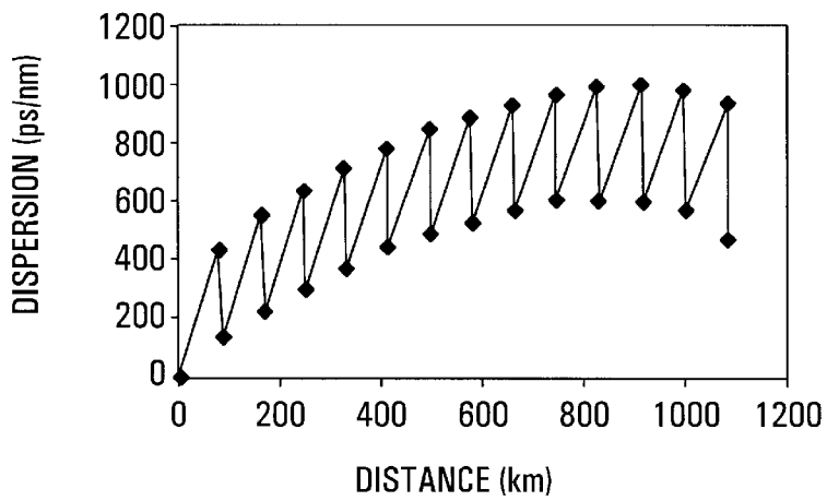
DISPERSION MAP WITH STATISTICAL VARIATIONS; TWC FIBER @1590nm
