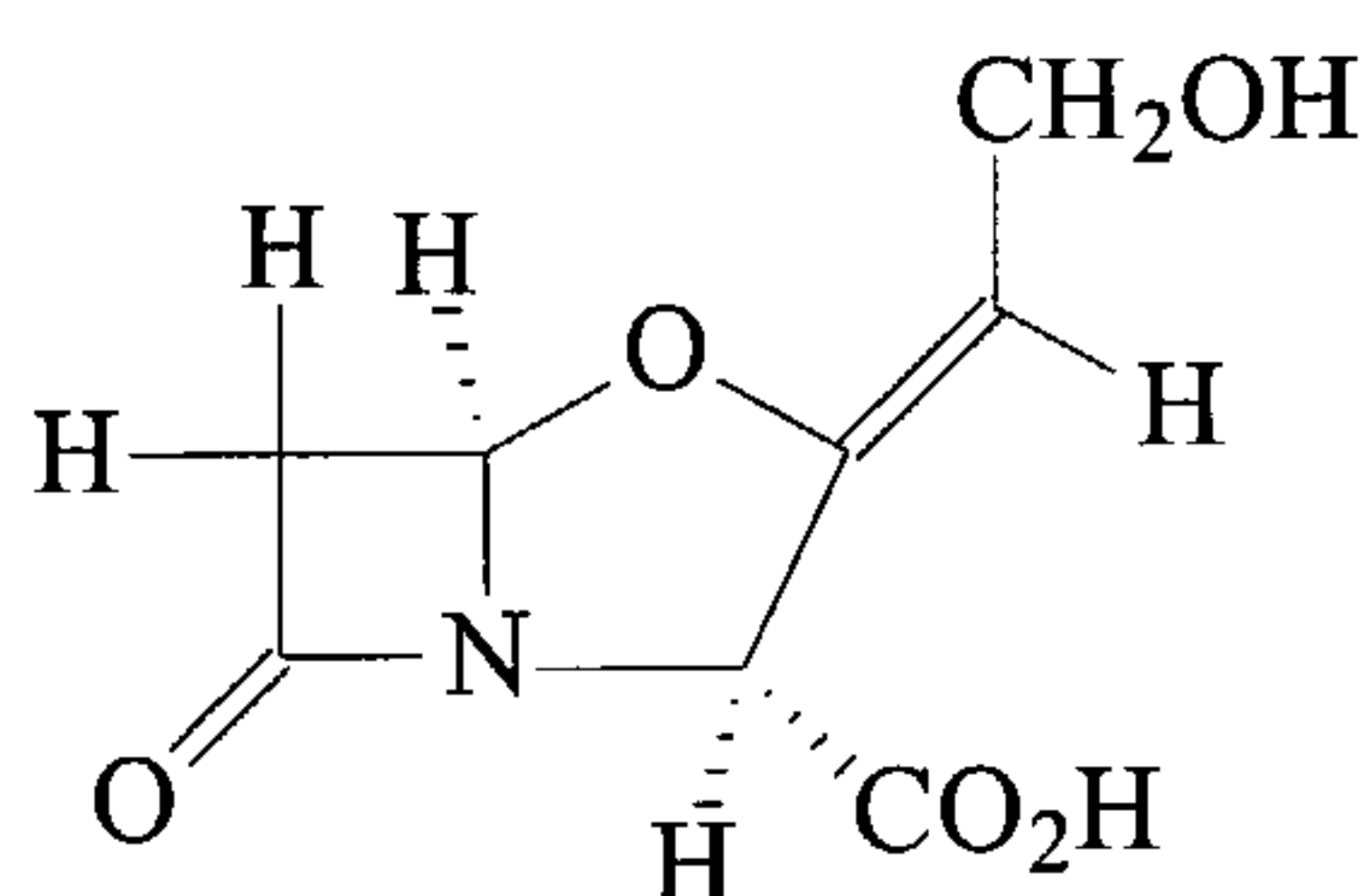
Clavulanic acid.
