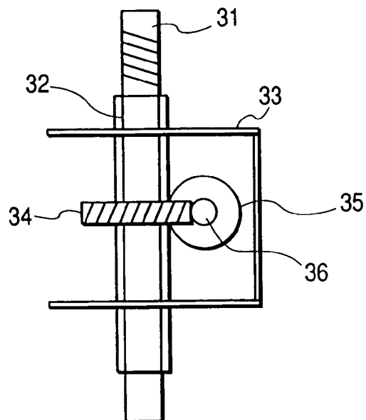
FIG. 3 (PRIOR ART)
