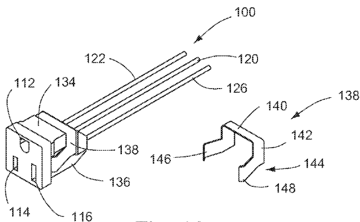
Fig. 16 (Prior Art)
