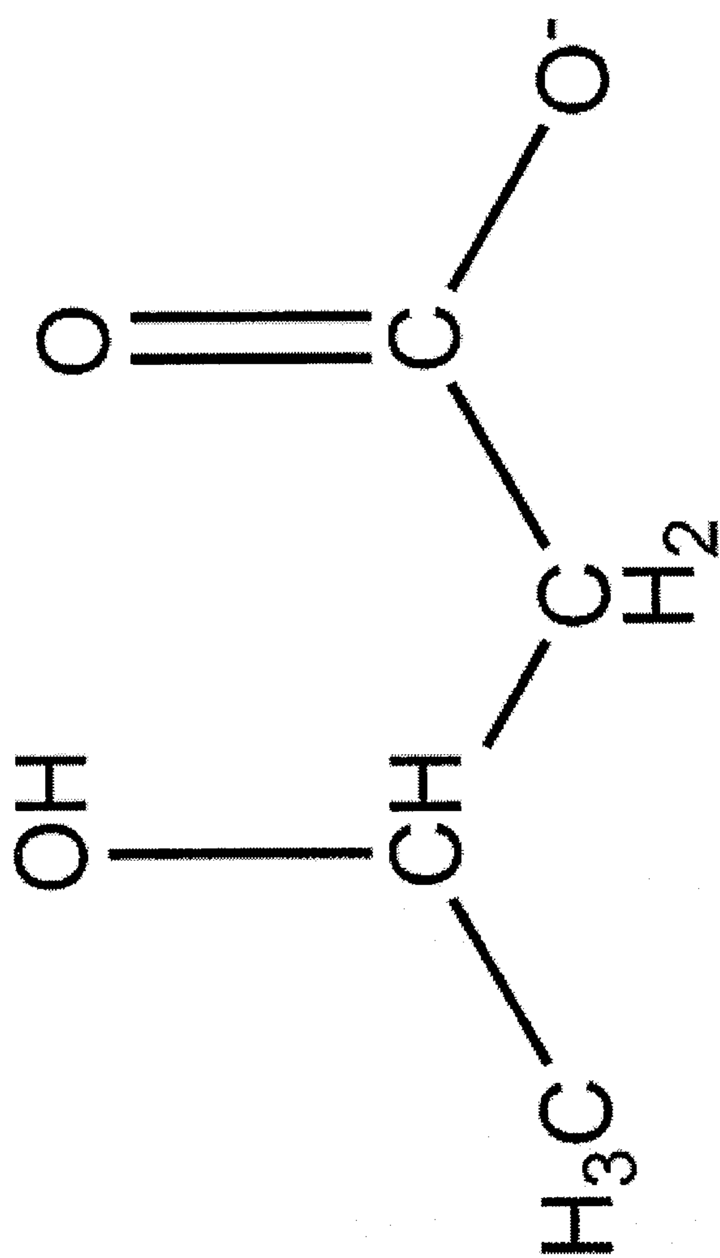
[2,4- 13 C]-β-hydroxybutyrate
