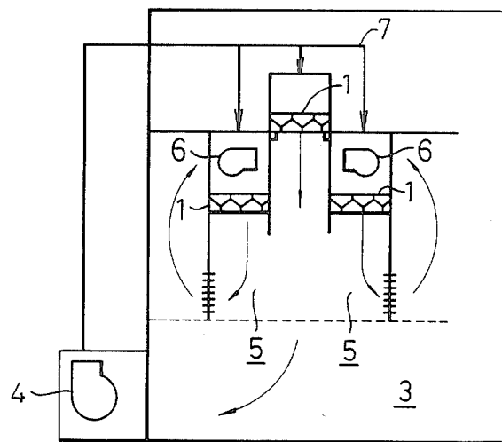
FIG. 2 (PRIOR ART)
