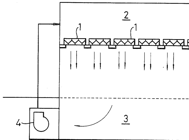
FIG. 1 (PRIOR ART)
