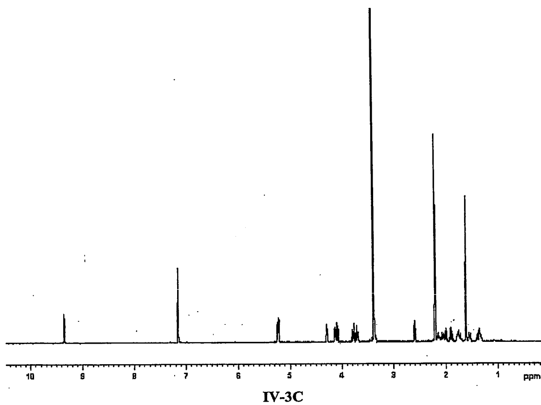
Figure 21. ^1\text{H} NMR spectrum of the compound of Formula IV-3C in \text{C}_6\text{D}_6/\text{DMSO-d}_6 .
