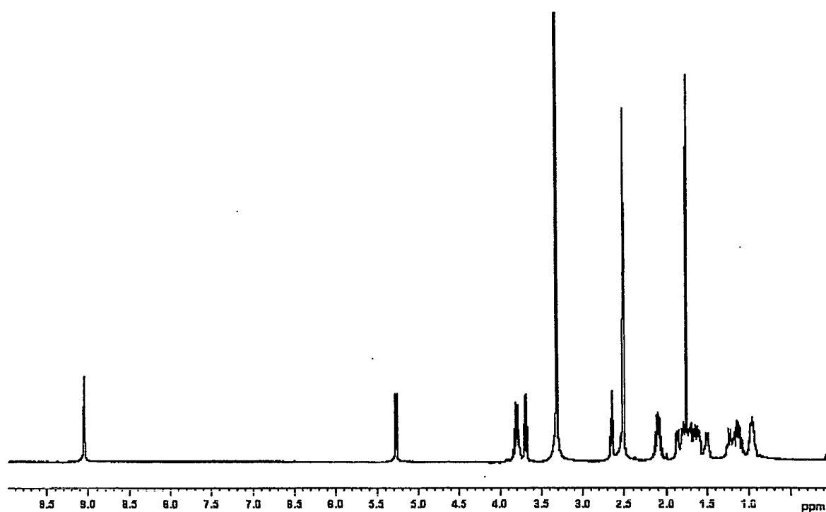
FIG. 14. ^1\text{H} NMR spectrum of compound of Formula II-4.
