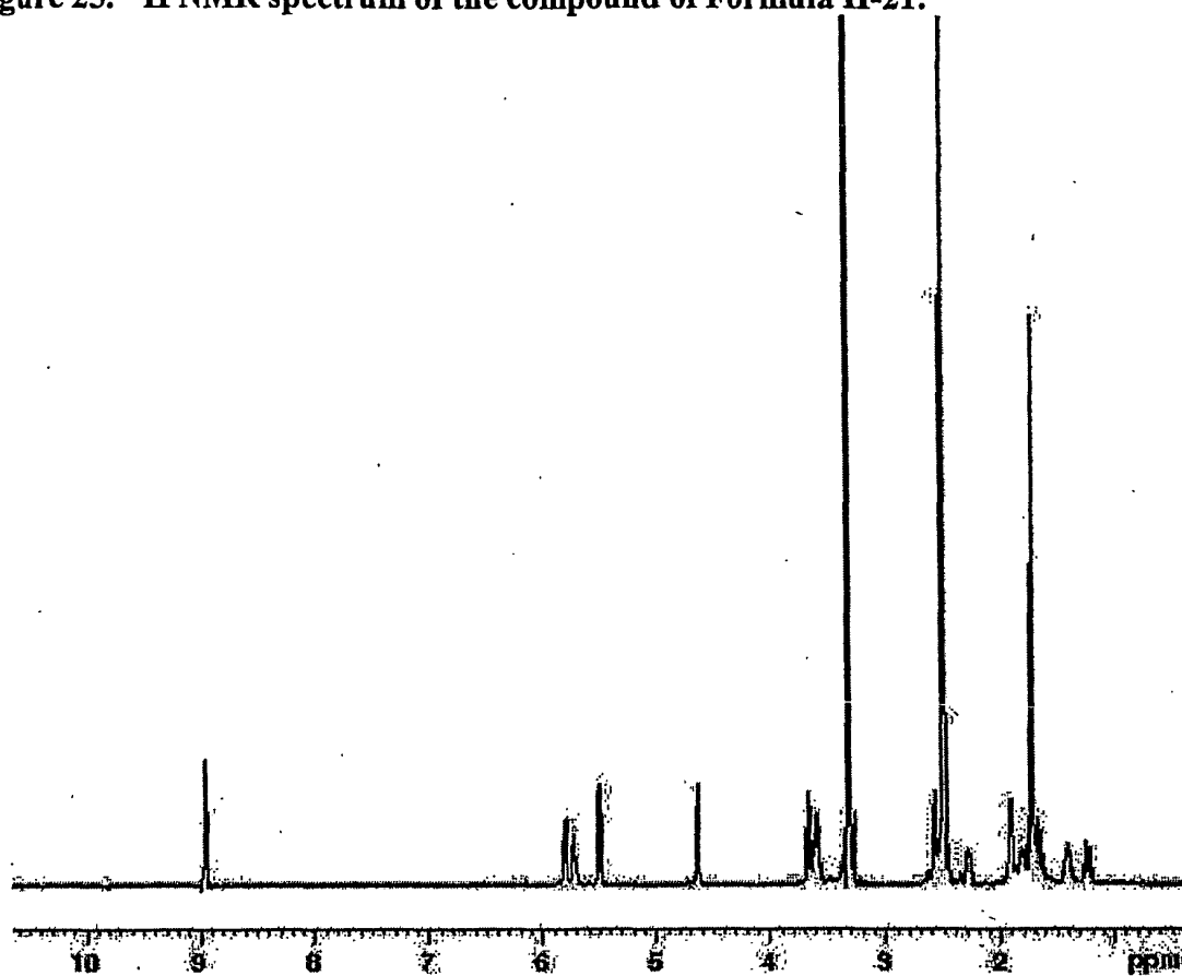
Figure 25. ^1\text{H} NMR spectrum of the compound of Formula II-21.
