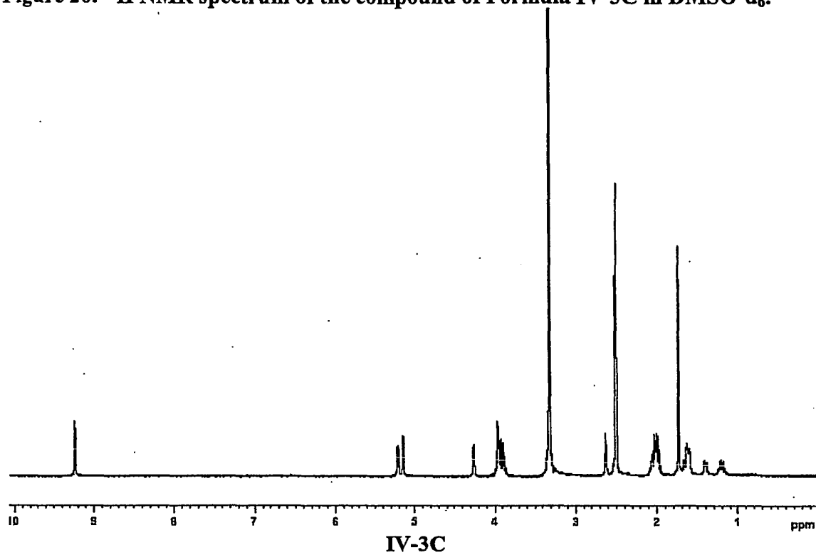
Figure 20. ^1\text{H} NMR spectrum of the compound of Formula IV-3C in \text{DMSO-d}_6 .
