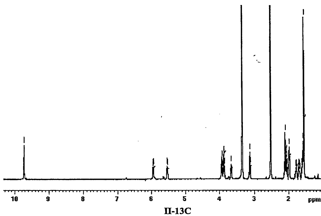
Figure 22. ^1\text{H} NMR spectrum of the compound of Formula II-13C.
