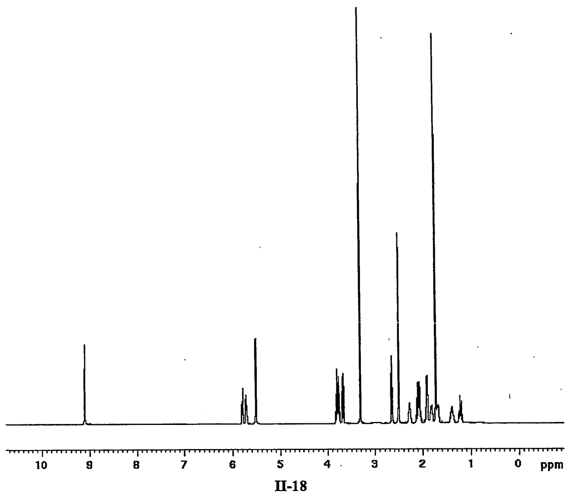
FIG. 50: ^1\text{H} NMR spectrum of the compound of Formula II-18.
