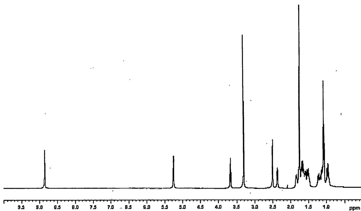
FIG. 12. ^1\text{H} NMR spectrum of compound of Formula II-3.
