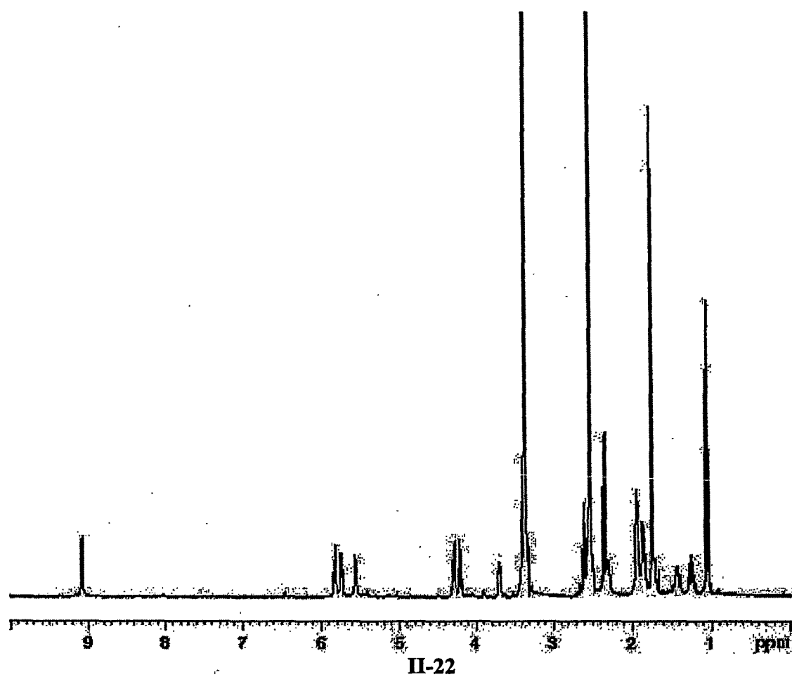
Figure 26. ^1\text{H} NMR spectrum of the compound of Formula II-22.
