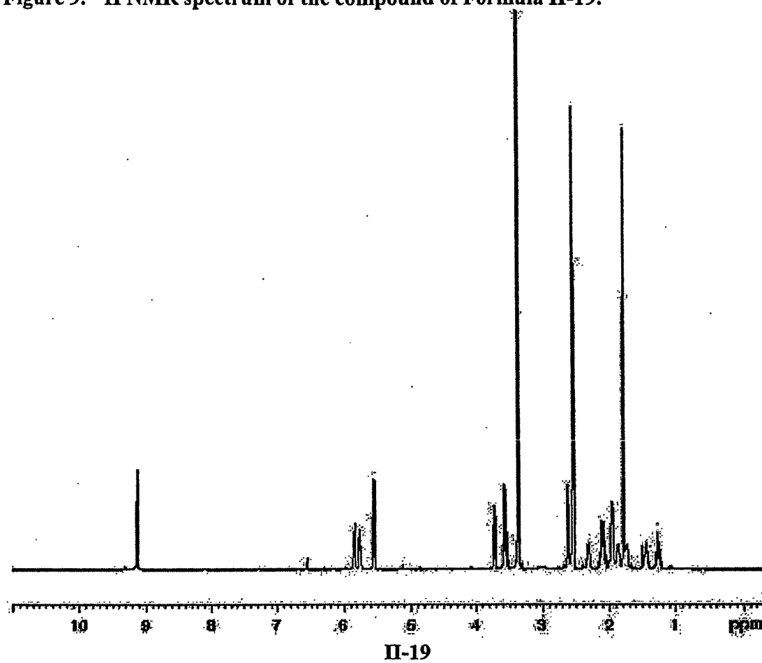
Figure 9. ^1\text{H} NMR spectrum of the compound of Formula II-19.
