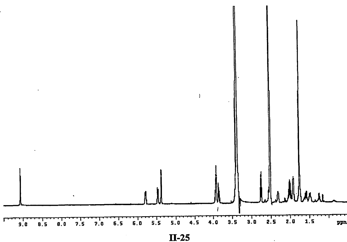
Figure 24. ^1\text{H} NMR spectrum of the compound of Formula II-25.
