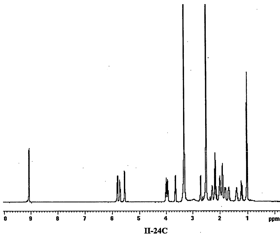
Figure 8. ^1\text{H} NMR spectrum of the compound of Formula II-24C.
