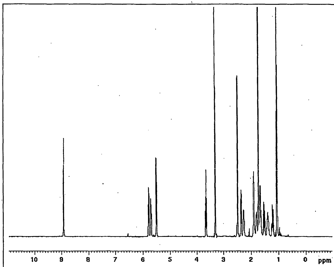
FIG. 49: ^1\text{H} NMR spectrum of the compound of Formula II-17.
