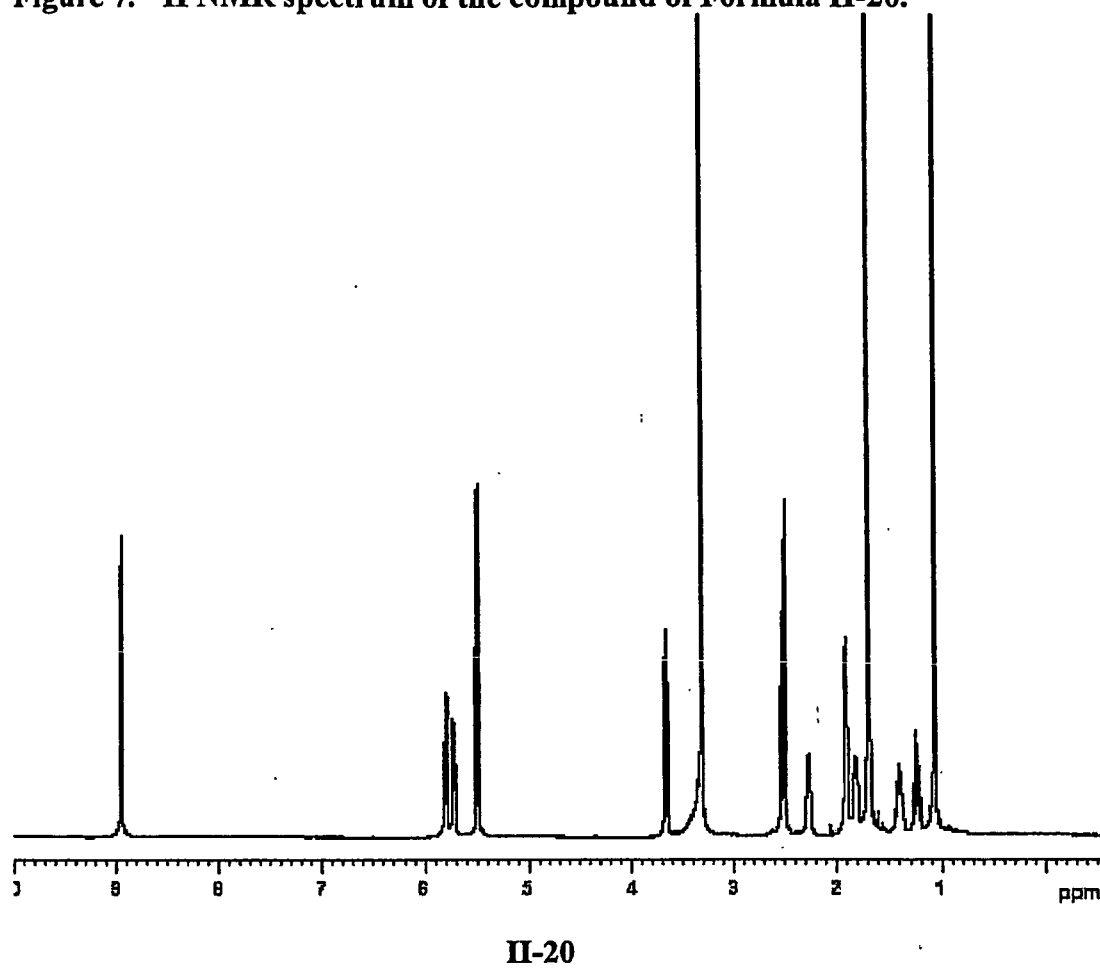
Figure 7. ^1\text{H} NMR spectrum of the compound of Formula II-20.
