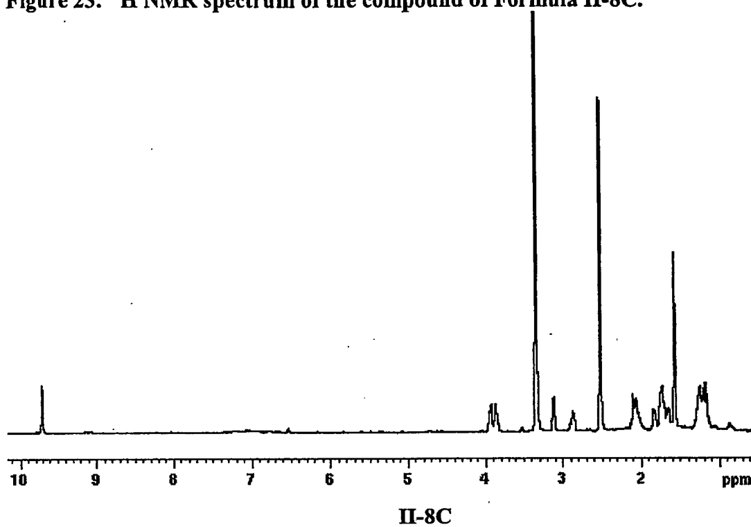
Figure 23. ^1\text{H} NMR spectrum of the compound of Formula II-8C.
