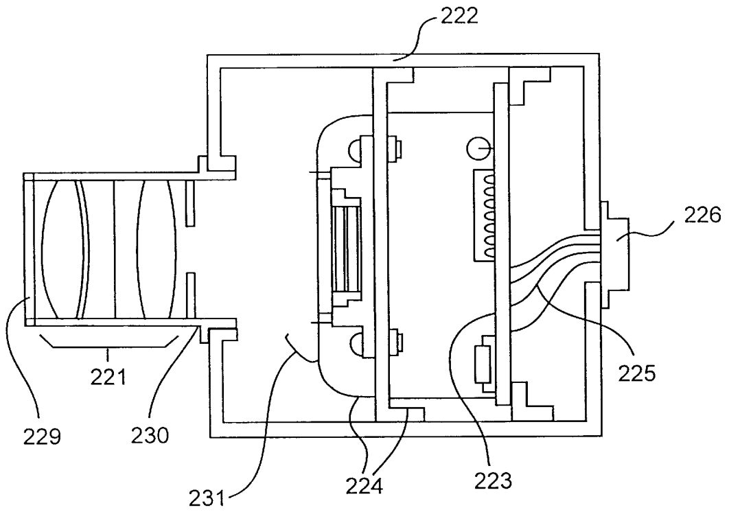
FIG. 9 PRIOR ART
