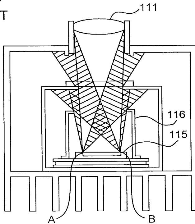
FIG. 10 PRIOR ART
