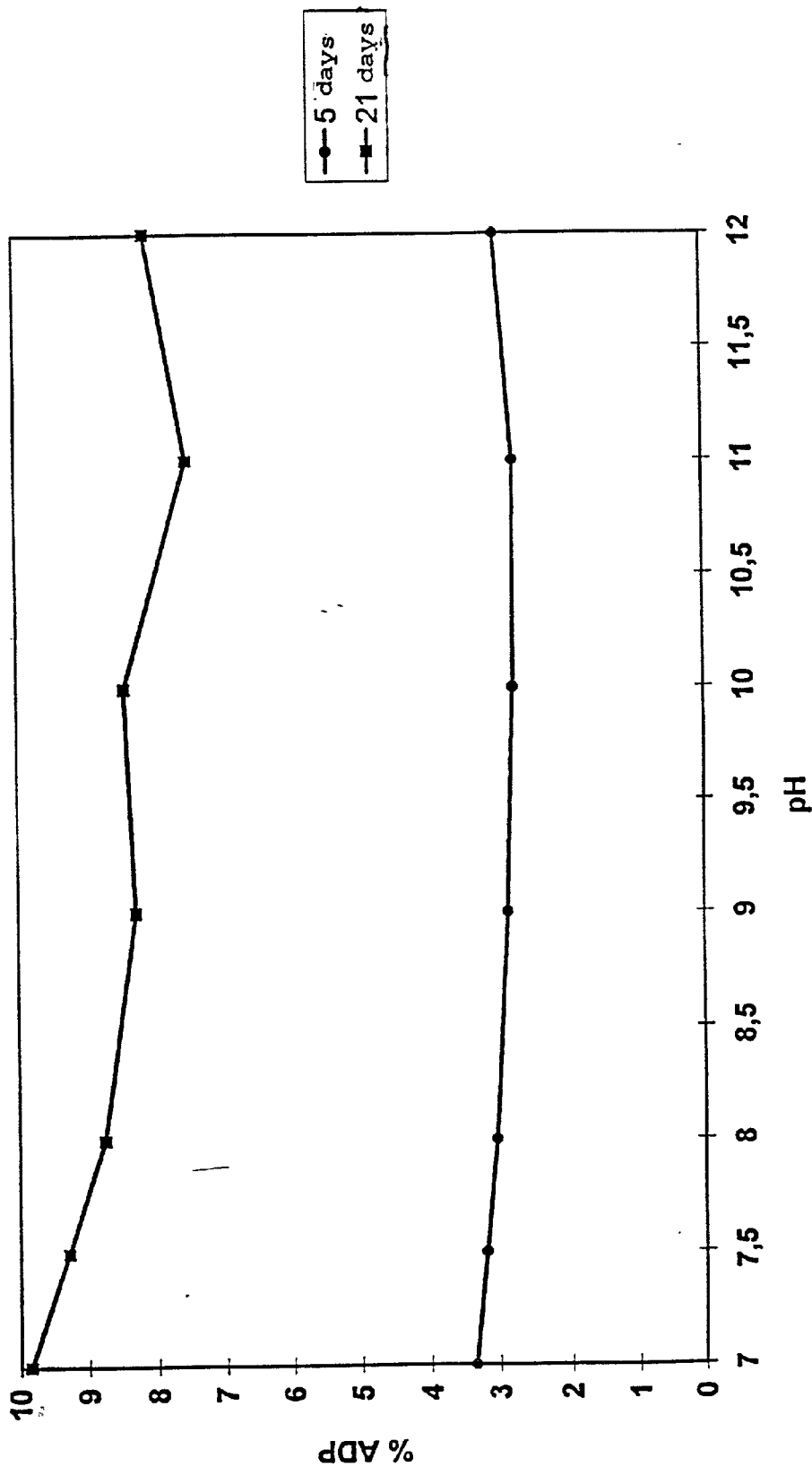
Fig. 10 stability ADP
