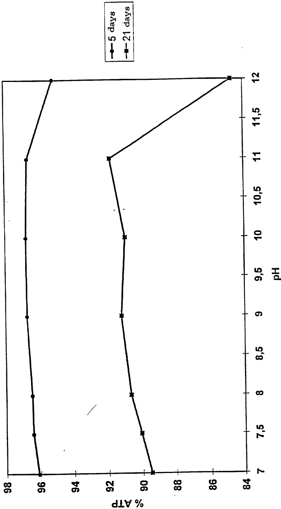
Fig. 9 stability ATP
