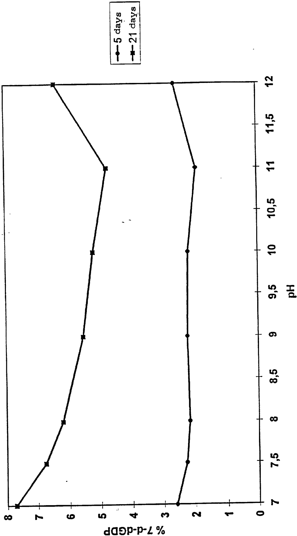
Fig. 12 stability 7-deaza-d-GTP
