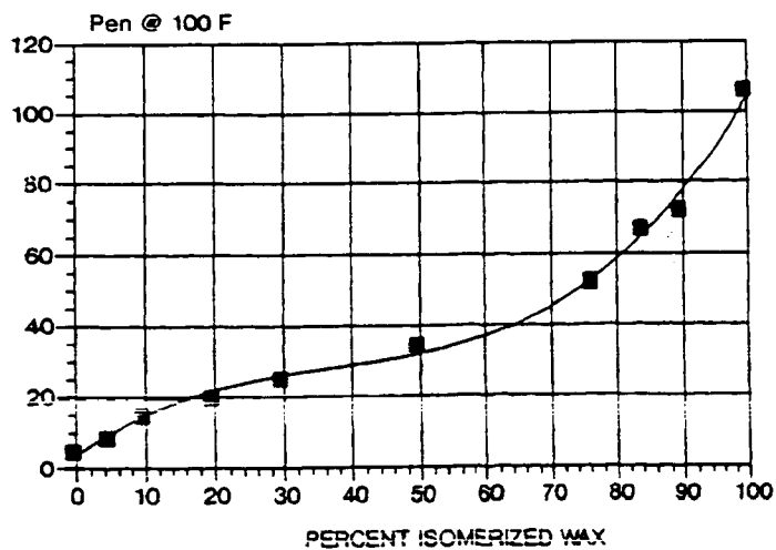
SOFTENING POINT INCREASED BY BLENDING ISOMERIZED WAX WITH RAW WAX
