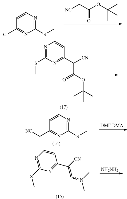
Reaction Scheme V
