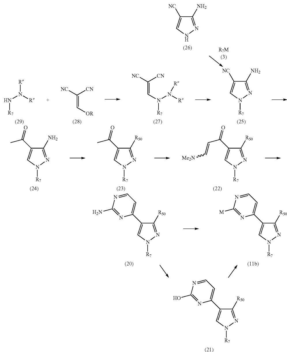
Reaction Scheme VI
