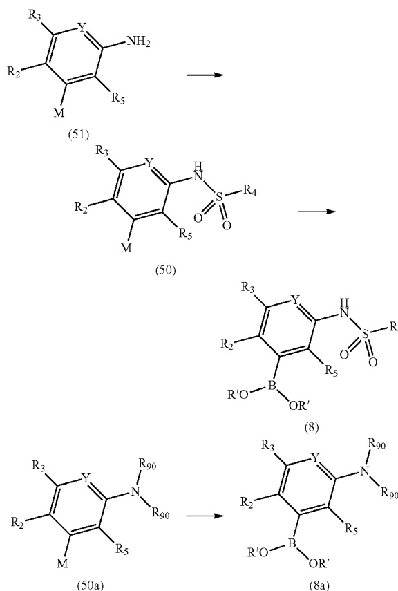
Reaction Scheme VII
