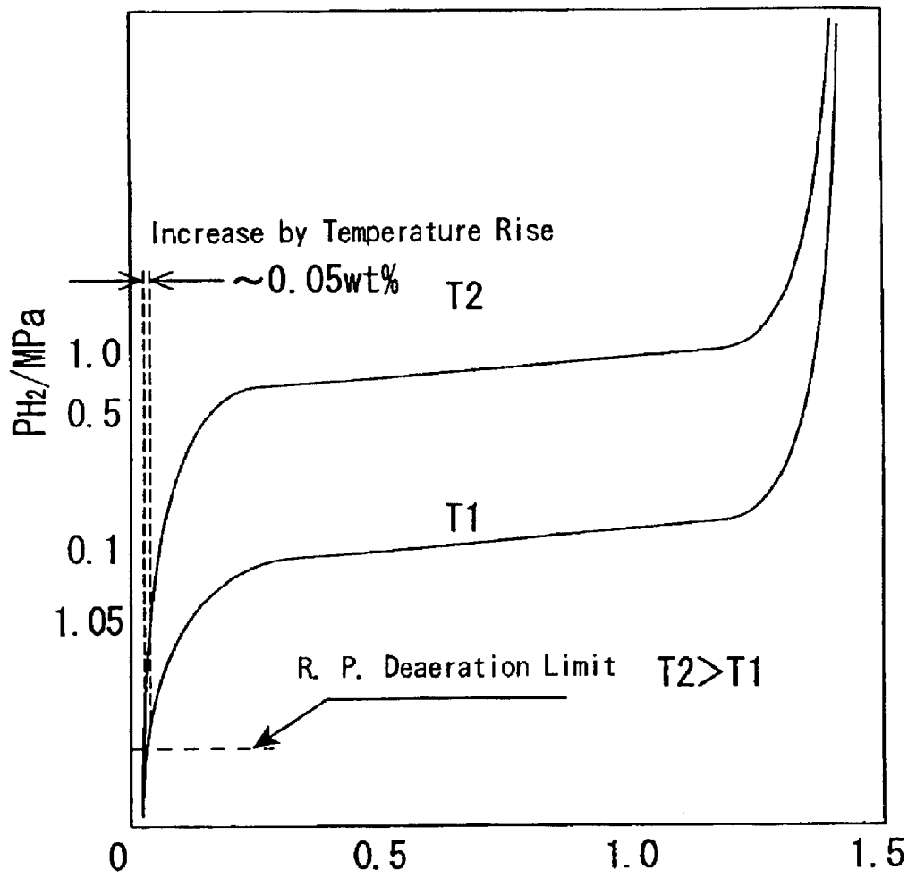
Changes in Hydrogen Release Amount by Temperature Rise upon Desorption of Hydrogen in a LaNi 5 System, etc.
