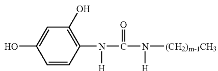
Structural Formula (8)
