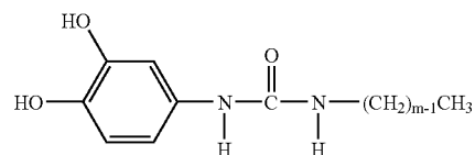
Structural Formula (5)
