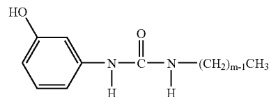
Structural Formula (4)
