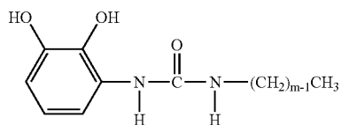
Structural Formula (7)
