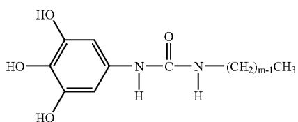
Structural Formula (8)
