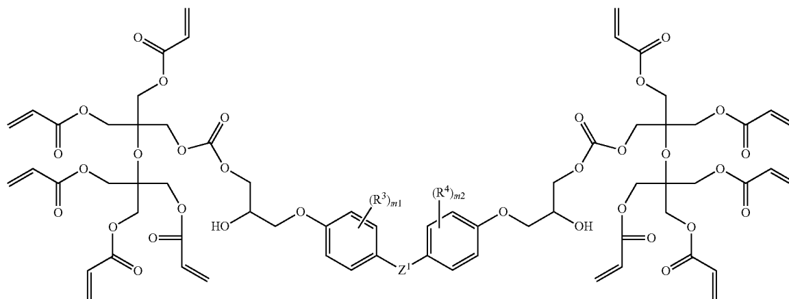
[Chemical Formula 8-2]
