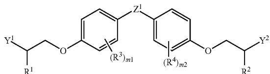
[Chemical Formula 2]
