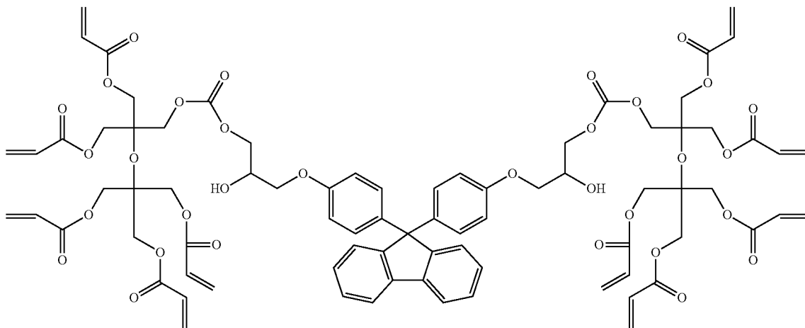
[Chemical Formula 13-2]
