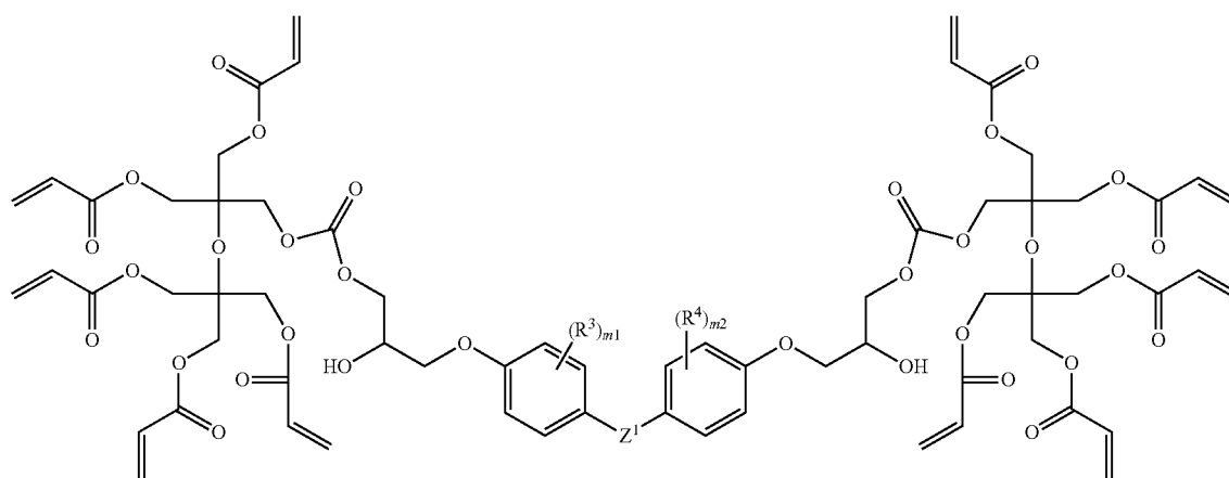
[Chemical Formula 8-3]
