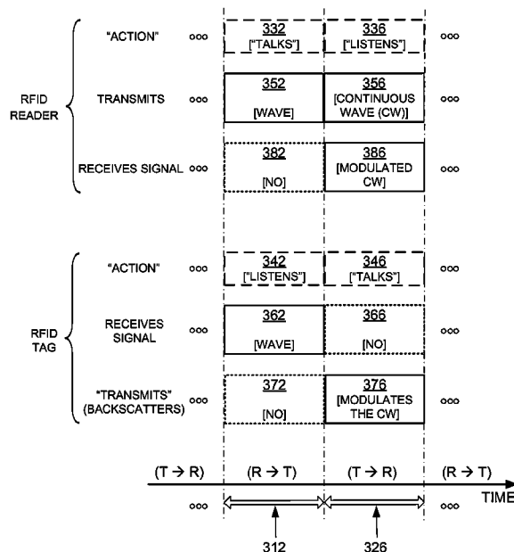
RFID SYSTEM COMMUNICATION
