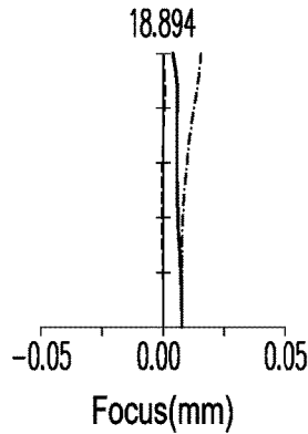
Field curvature (sagittal direction) HFOV (°)
