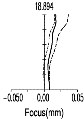
Field curvature (tangential direction) HFOV (°)
