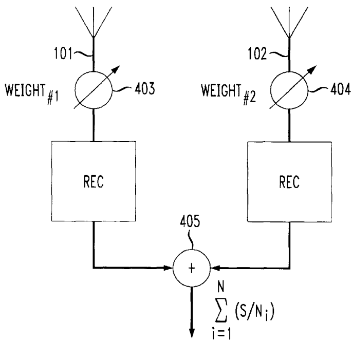
FIG. 4C MAXIMAL-RATIO COMBINING
