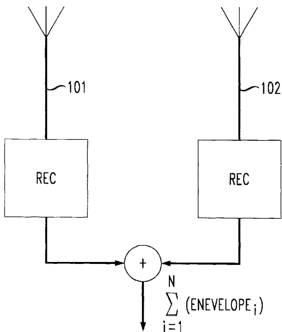
FIG. 4D EQUAL-GAIN COMBINING
