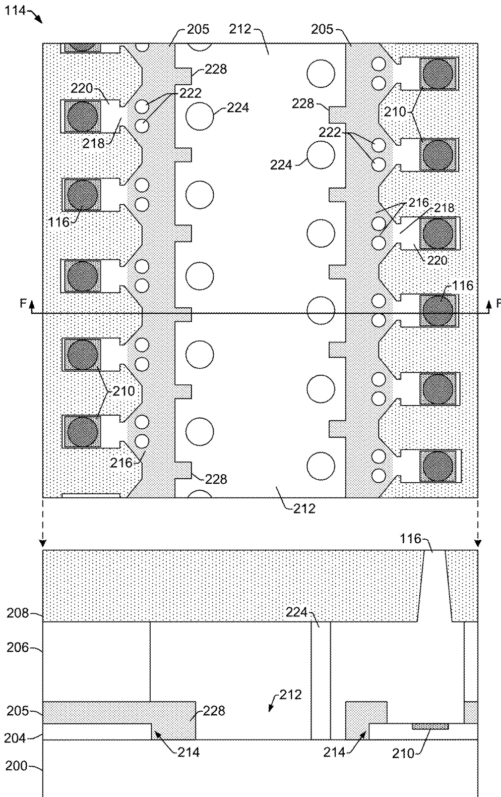
View F-F
