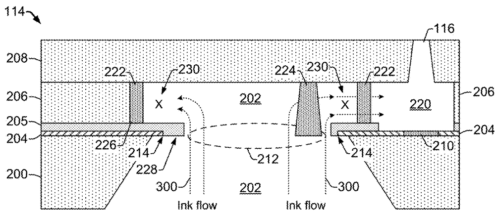
View A-A from FIG. 2
