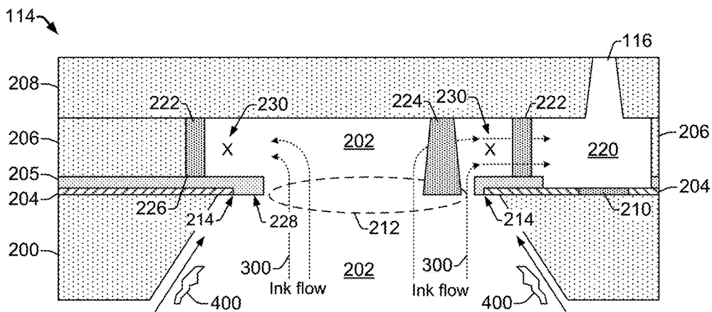
View B-B from FIG. 2
