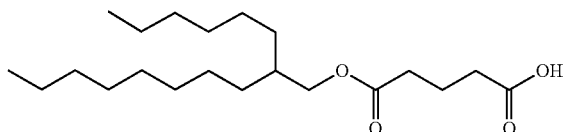
Synthesis of 5-(2-hexyldecoxy)-5-oxo-pentanoic acid
