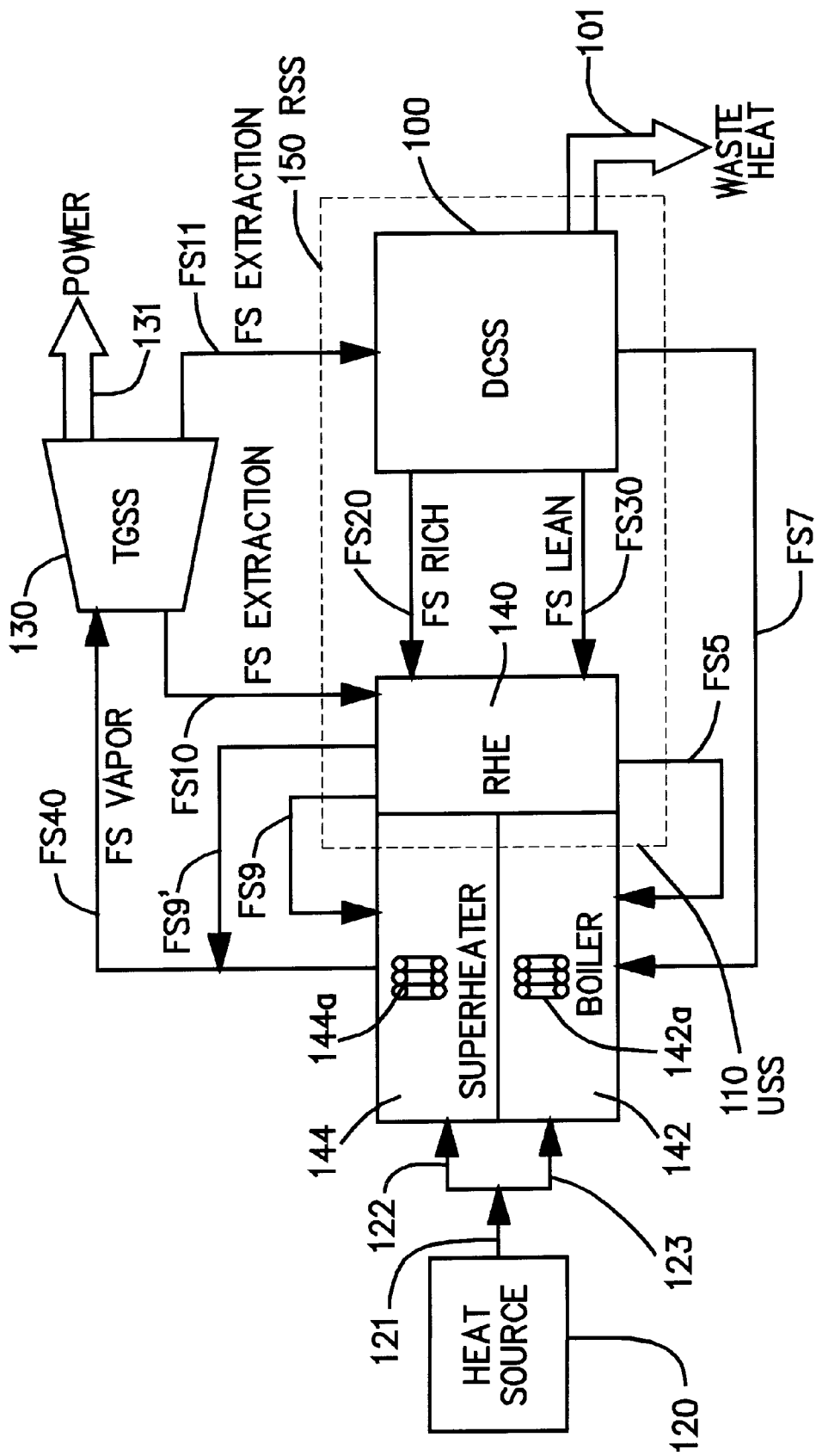
Figure 1 (PRIOR ART)
