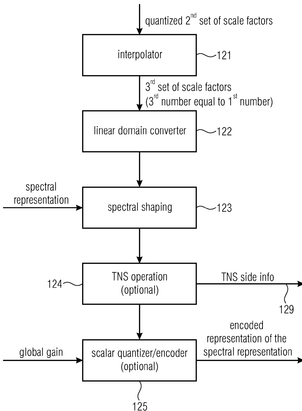
Fig. 5 (SPECTRAL PROCESSOR)
