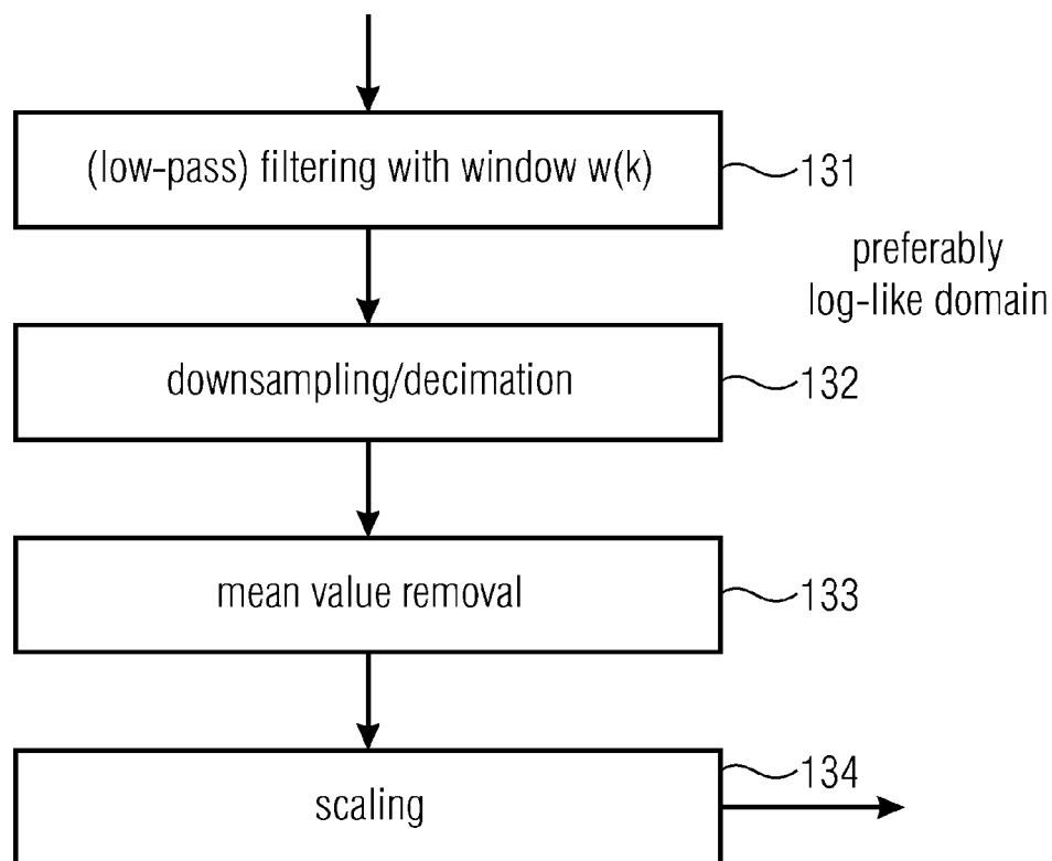
Fig. 3 (DOWNSAMPLER)
