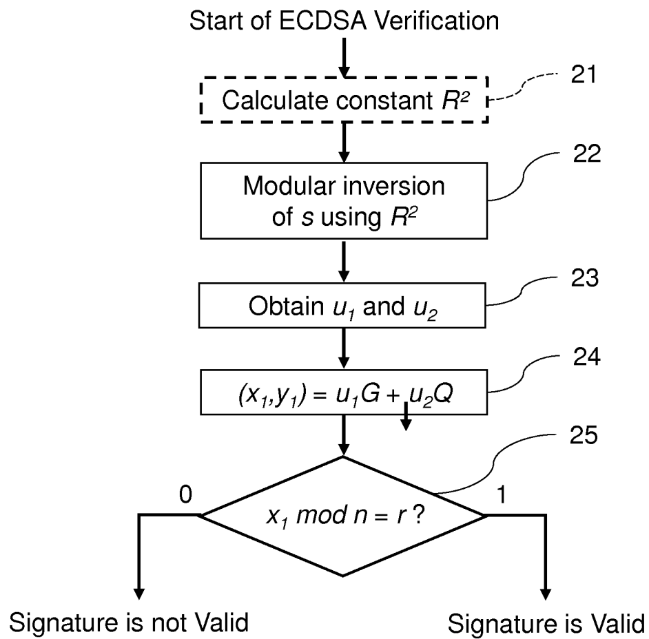
FIG.2 PRIOR ART
