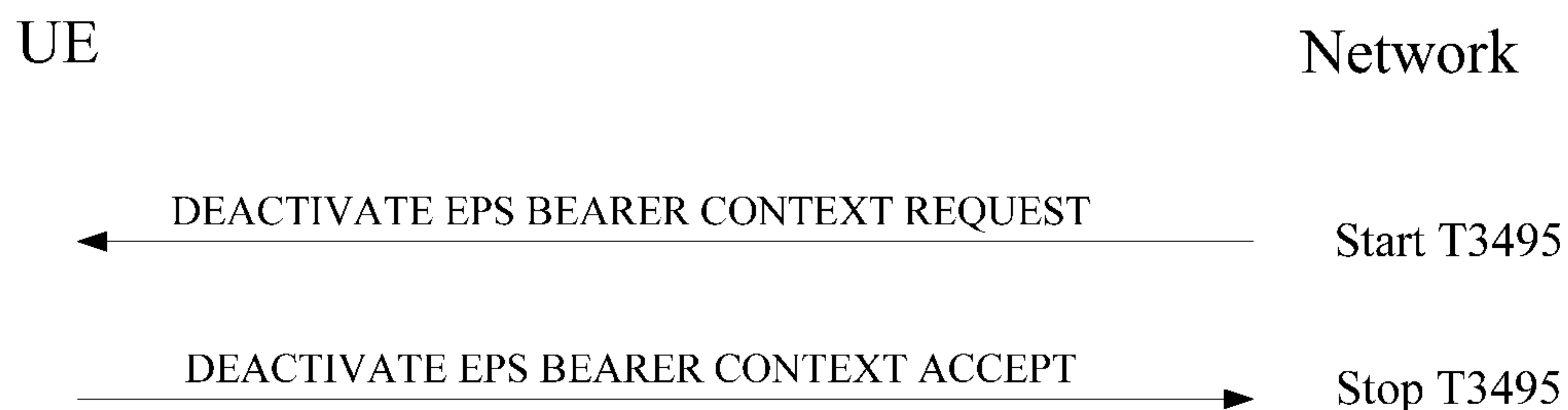
Figure 6.4.4.2.1: EPS bearer context deactivation procedure
