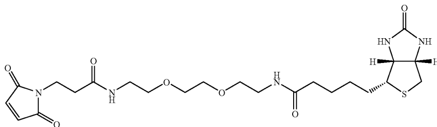
Biotin-PEO-maleimide
