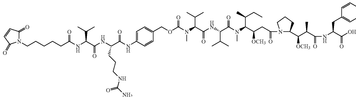
MC-val-cit-PAB-MMAF
