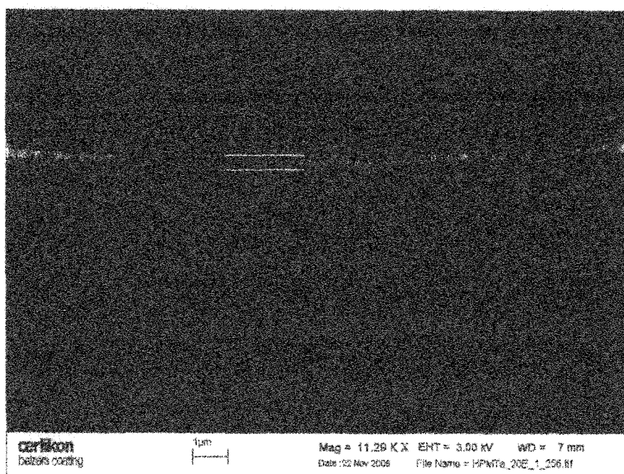
Fig.8 (process ID: HPMTa_20c) 180W RF bias. 2.0 \mu\text{m} top thickness, 410 nm bottom thickness, 21% bottom coverage.
