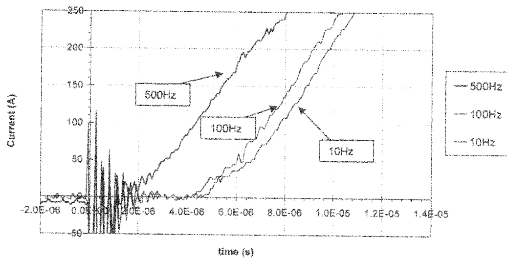
FIG. 2 Experiment: current pulse rise time as function of frequency. (upper graph: 500 Hz, middle: 100 Hz; bottom: 10 Hz)
