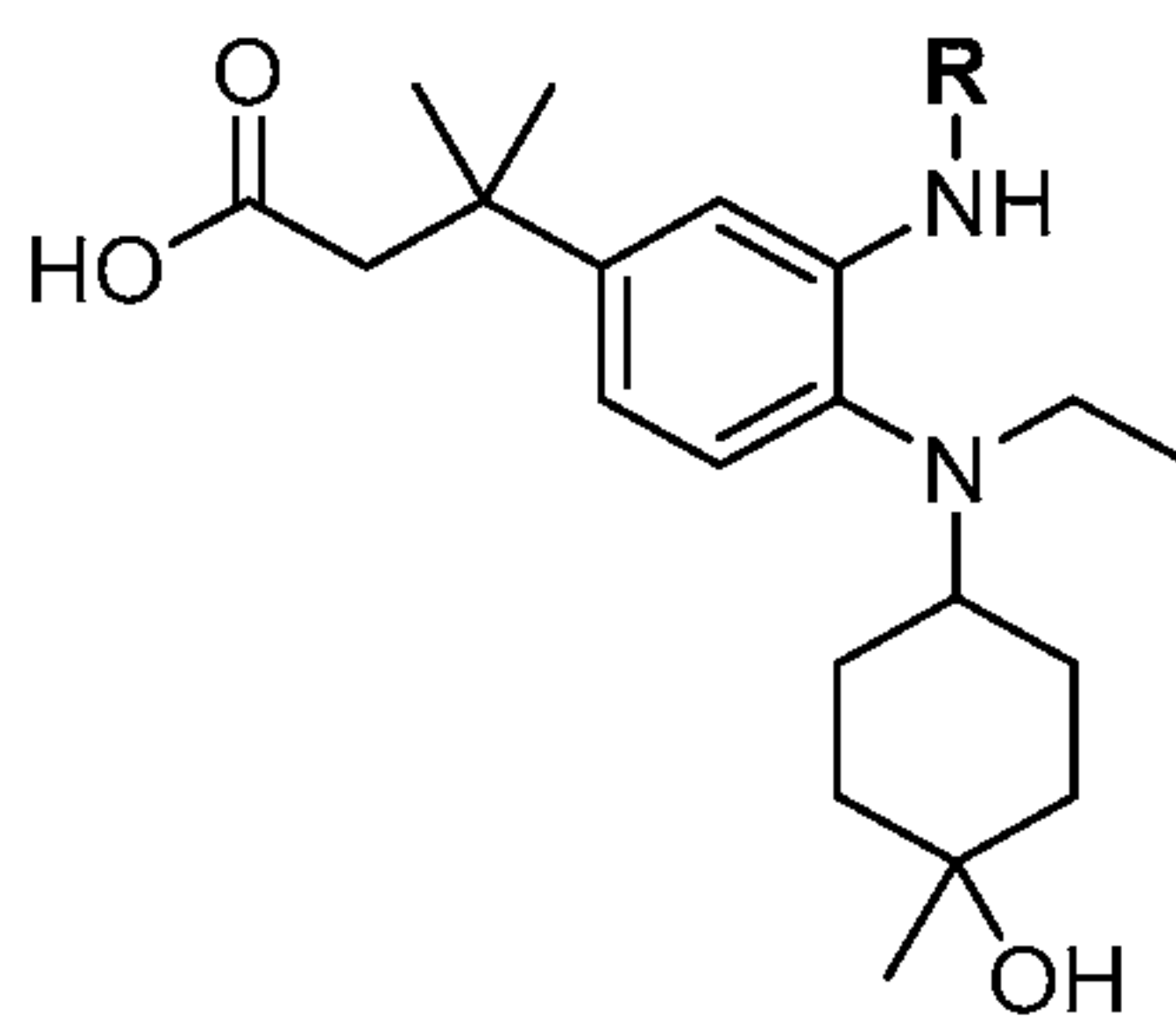
Examples 2 to 4
