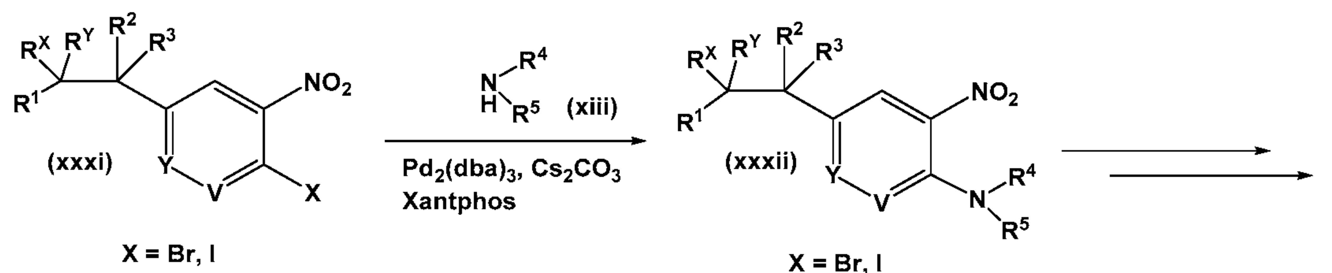
Scheme 9
