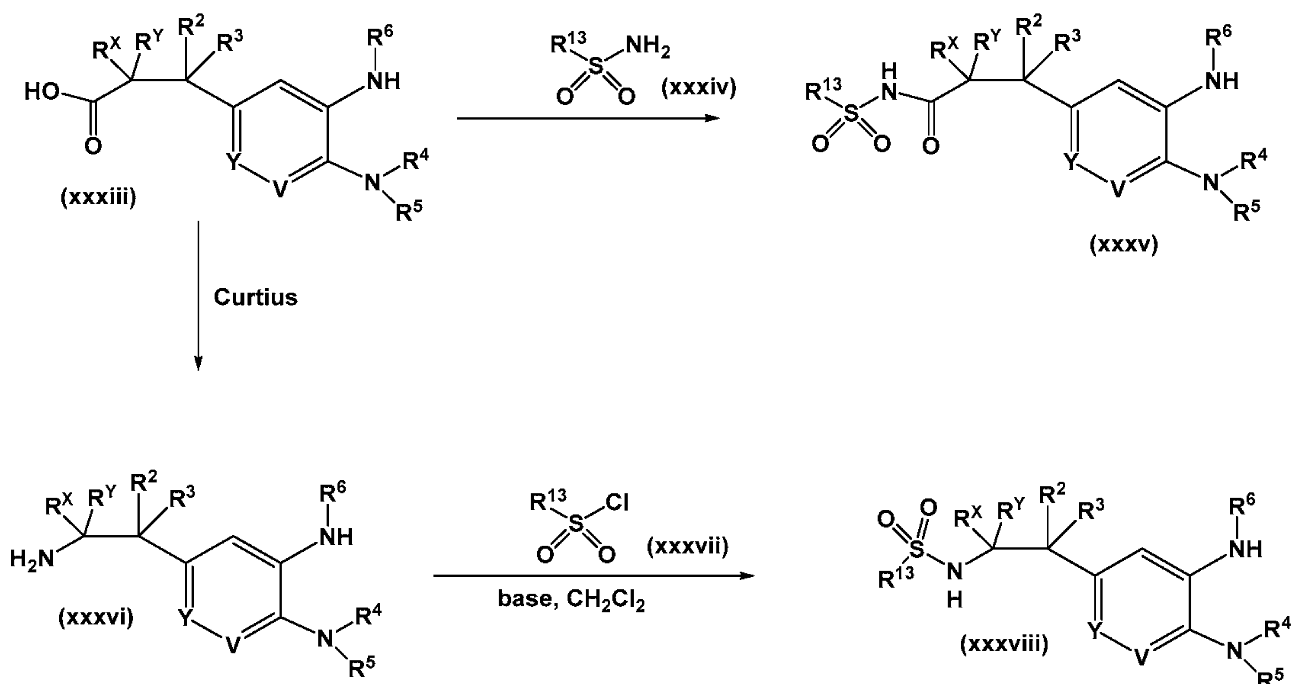
Scheme 10
