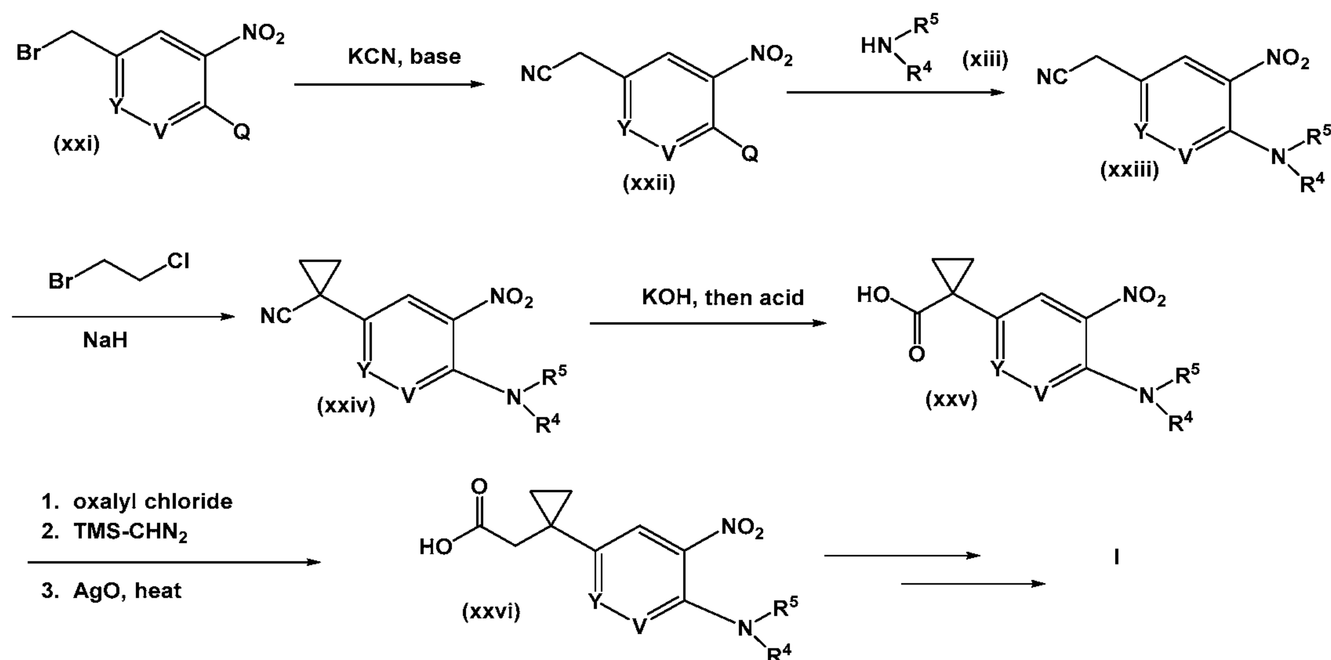
Scheme 6
