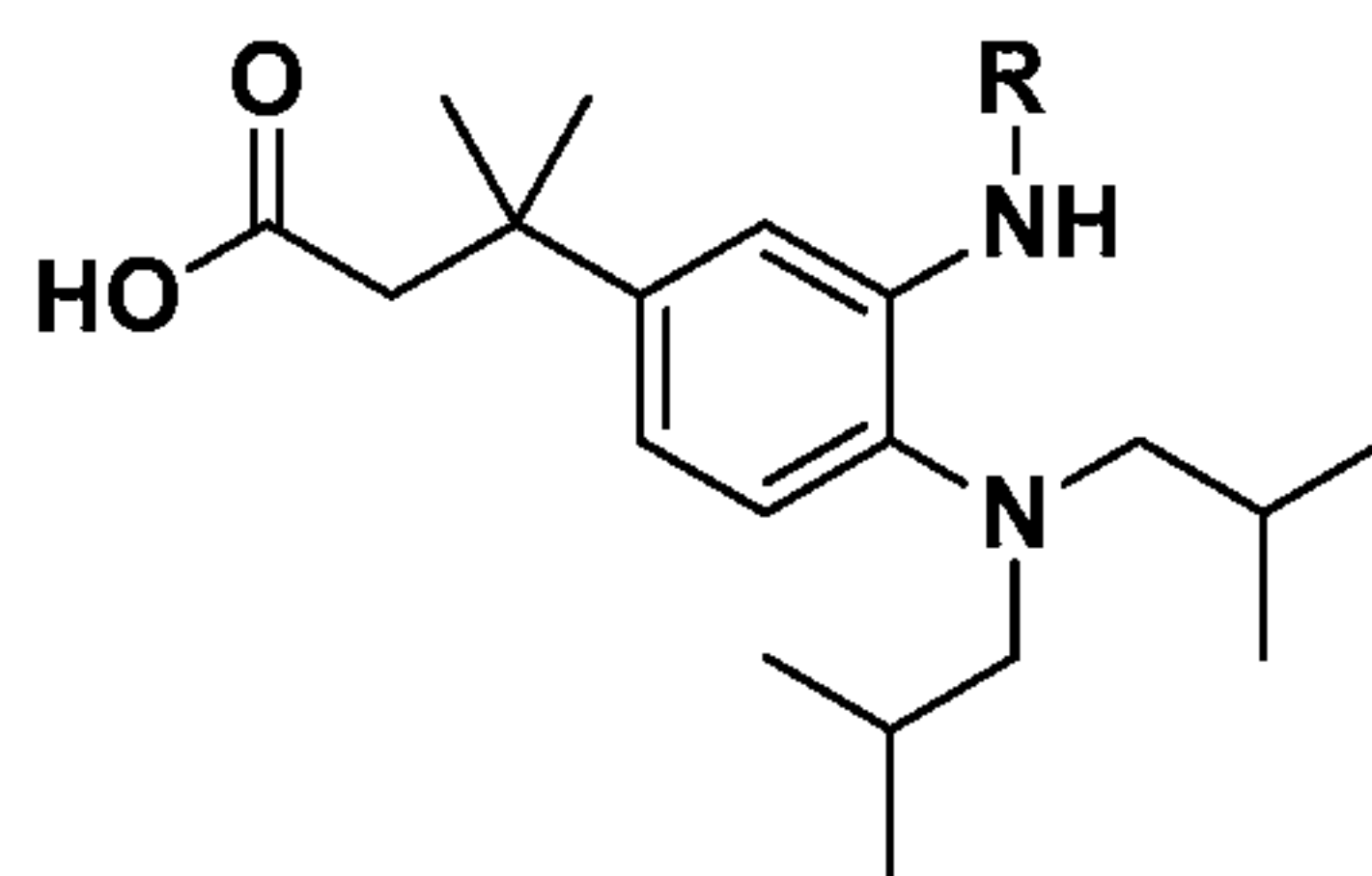
Examples 146 to 148
