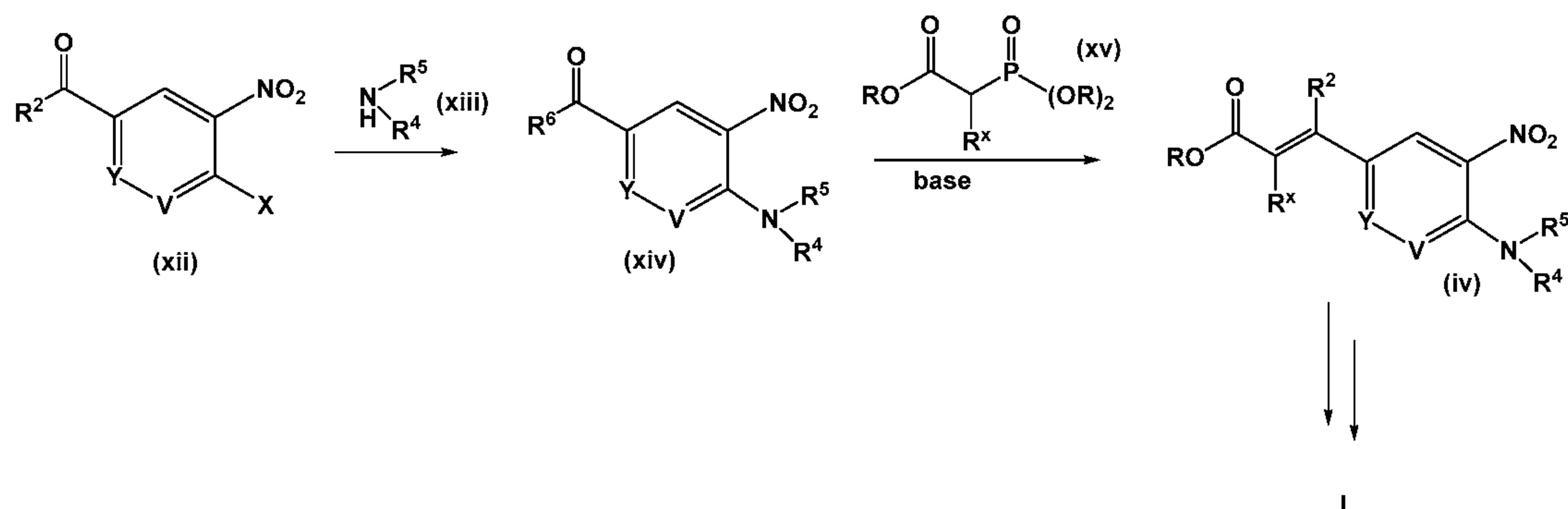
Scheme 3
