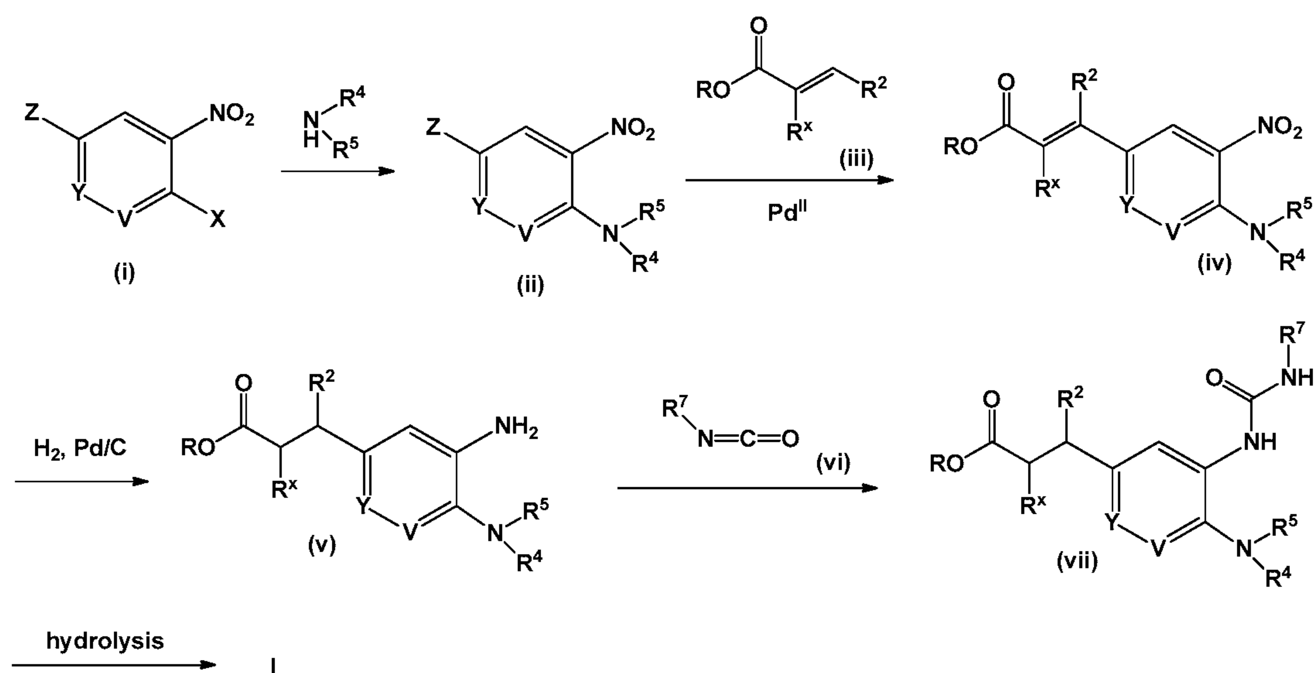
Scheme 1
