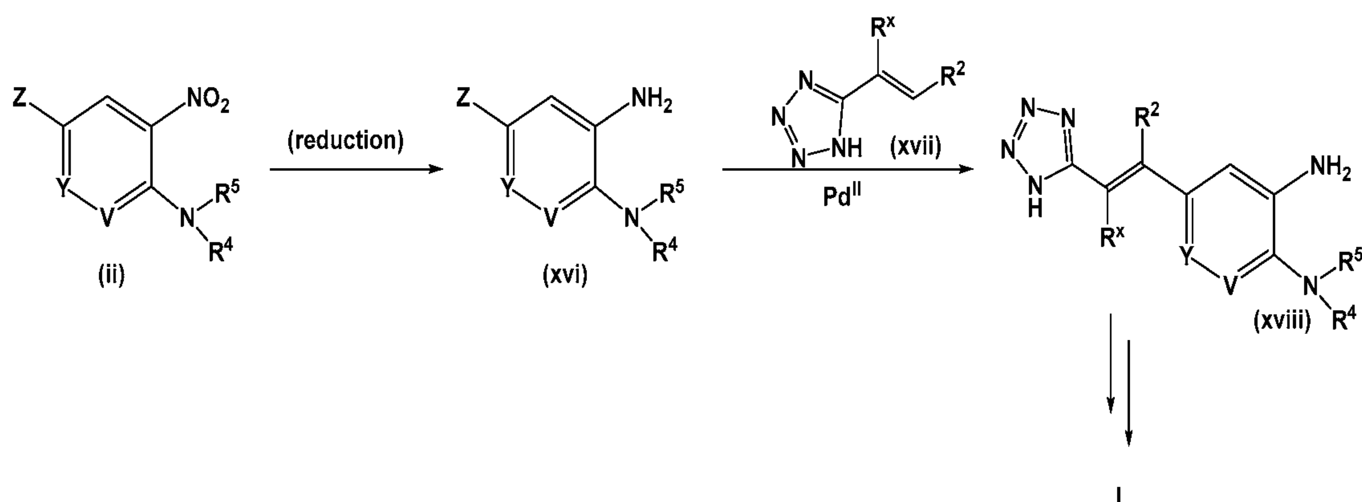
Scheme 4
