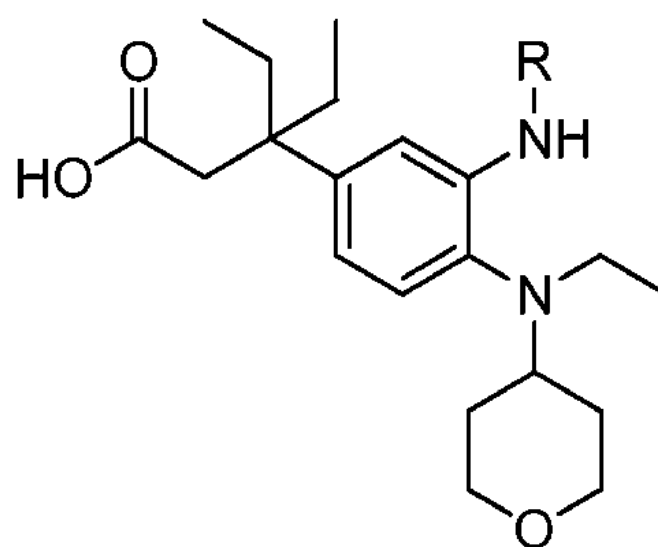
Examples 27 to 29
