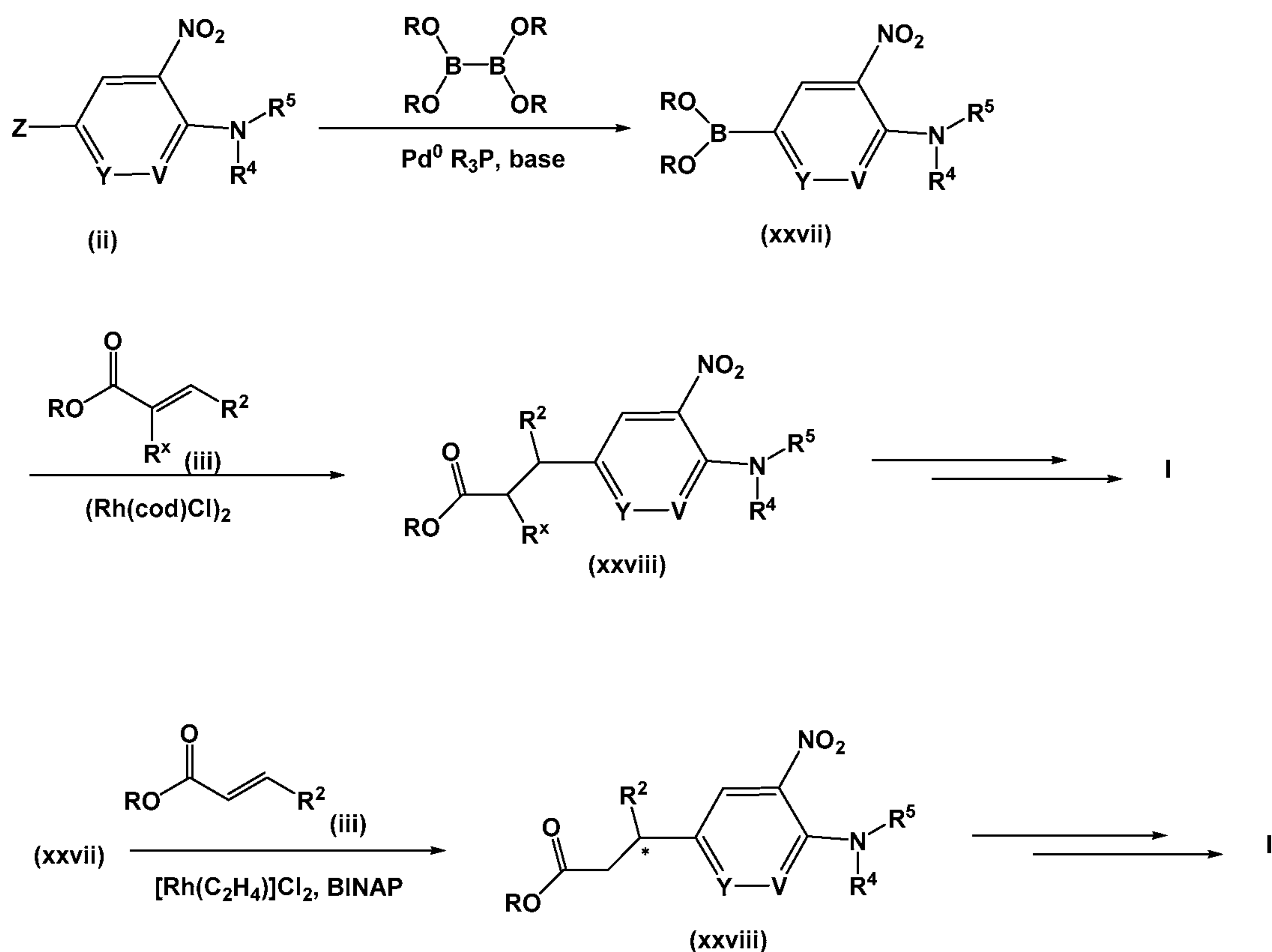
Scheme 7
