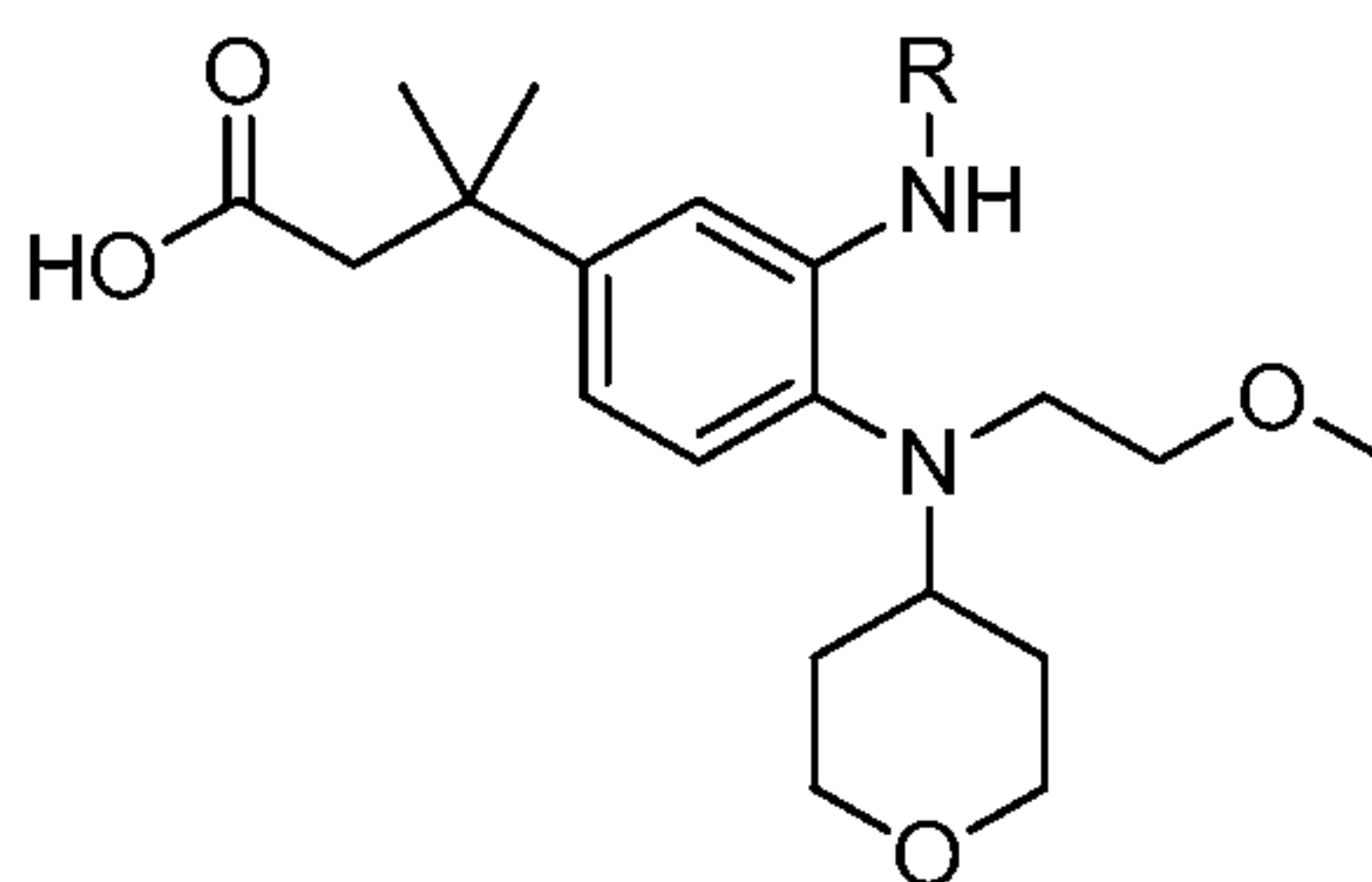
Examples 16 and 17
