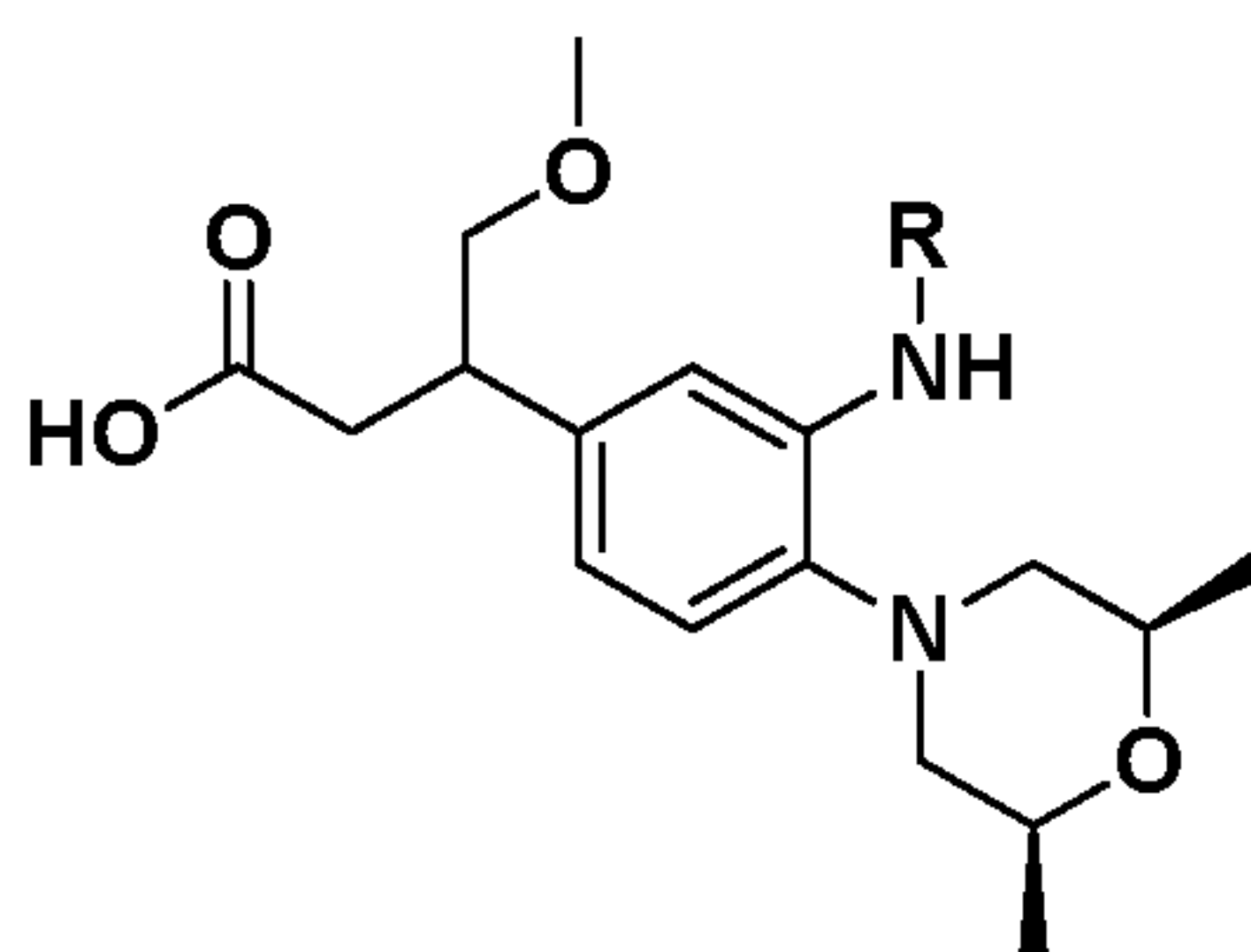
Example 603 (Diastereomer 1)
