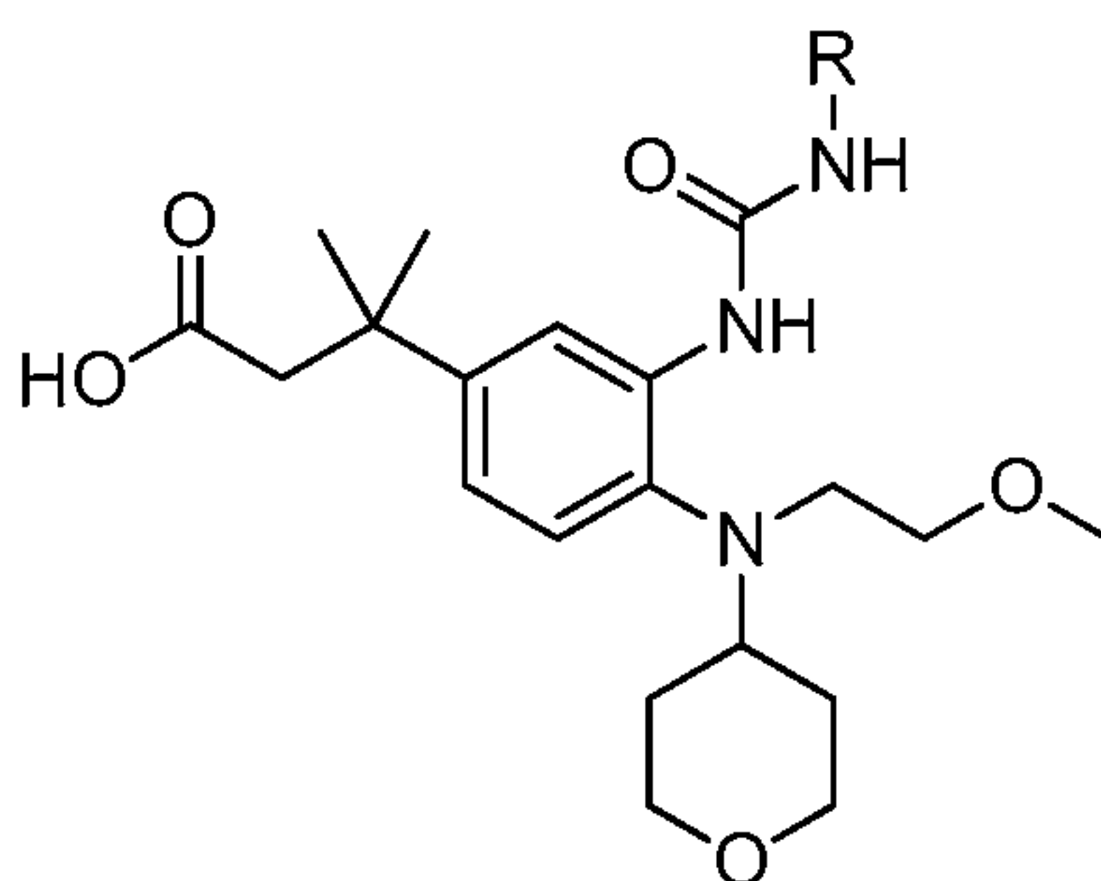
Examples 19 and 20
