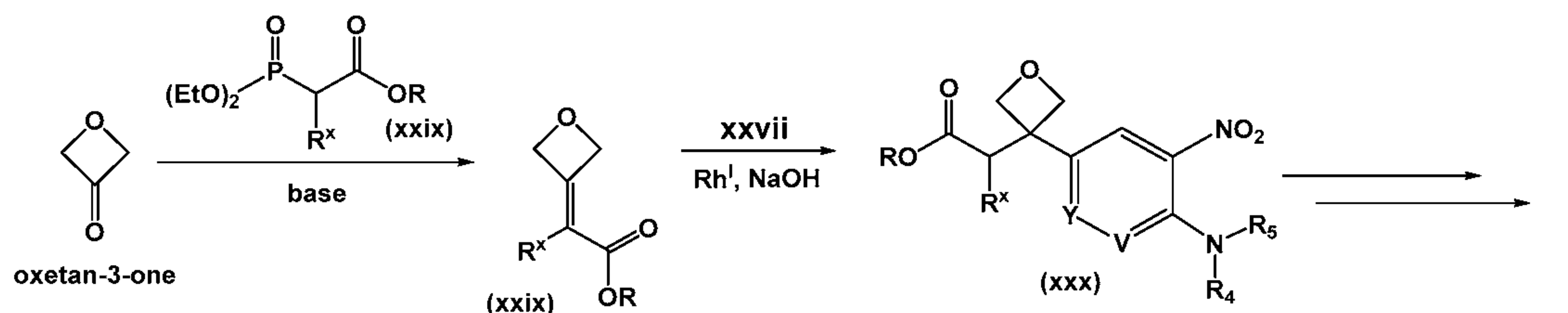
Scheme 8
