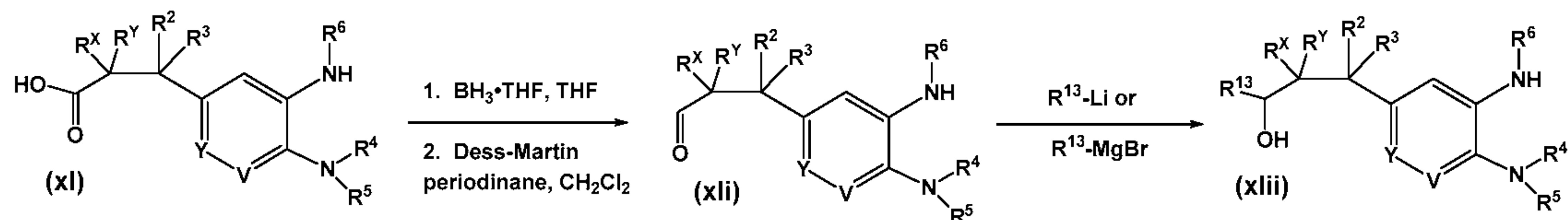
Scheme 11
