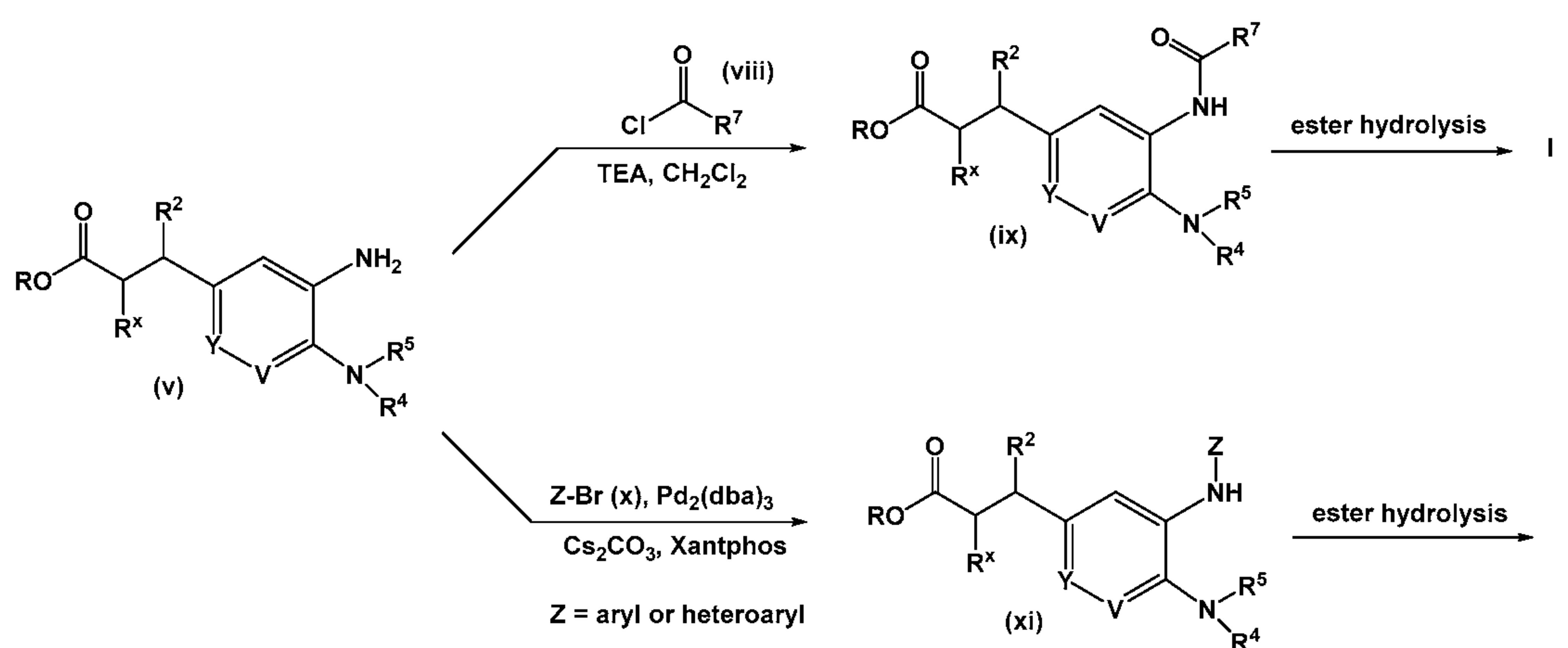
Scheme 2
