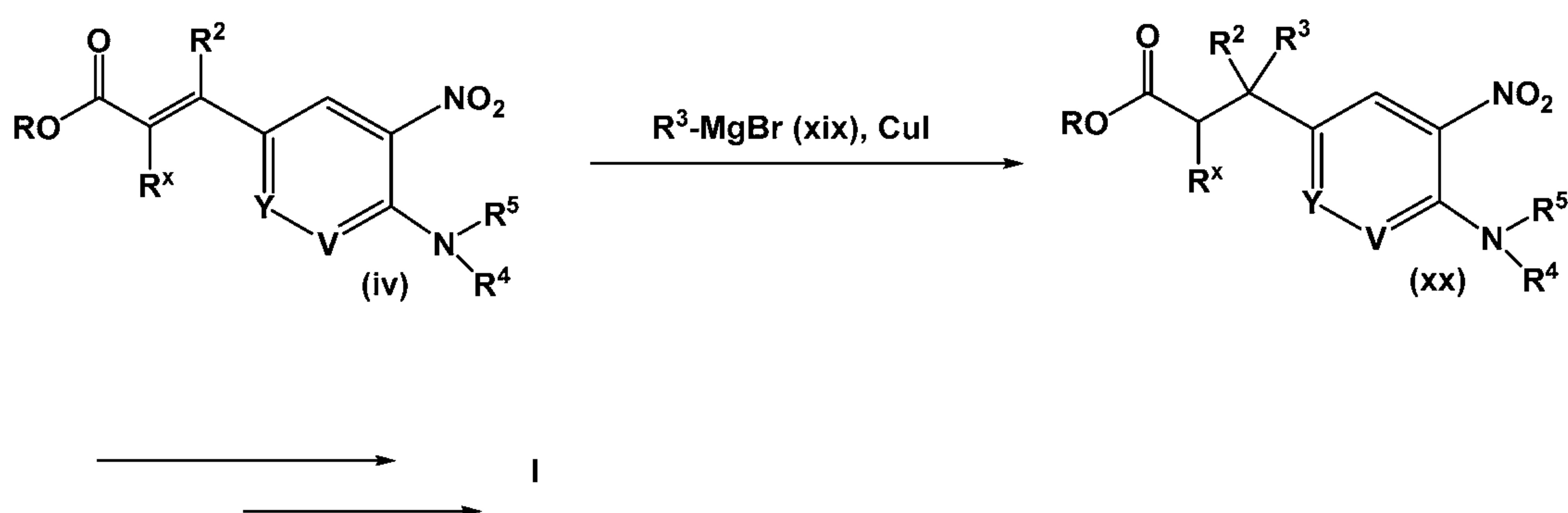
Scheme 5
