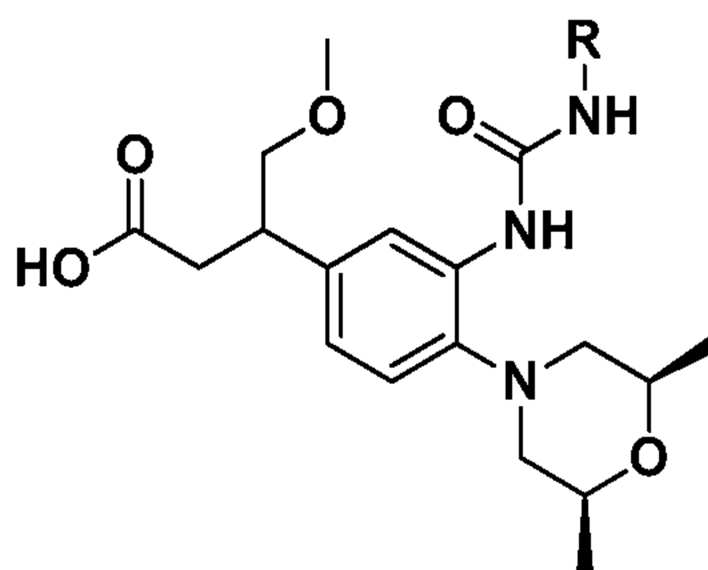
Example 606 (Diastereomer 1)
