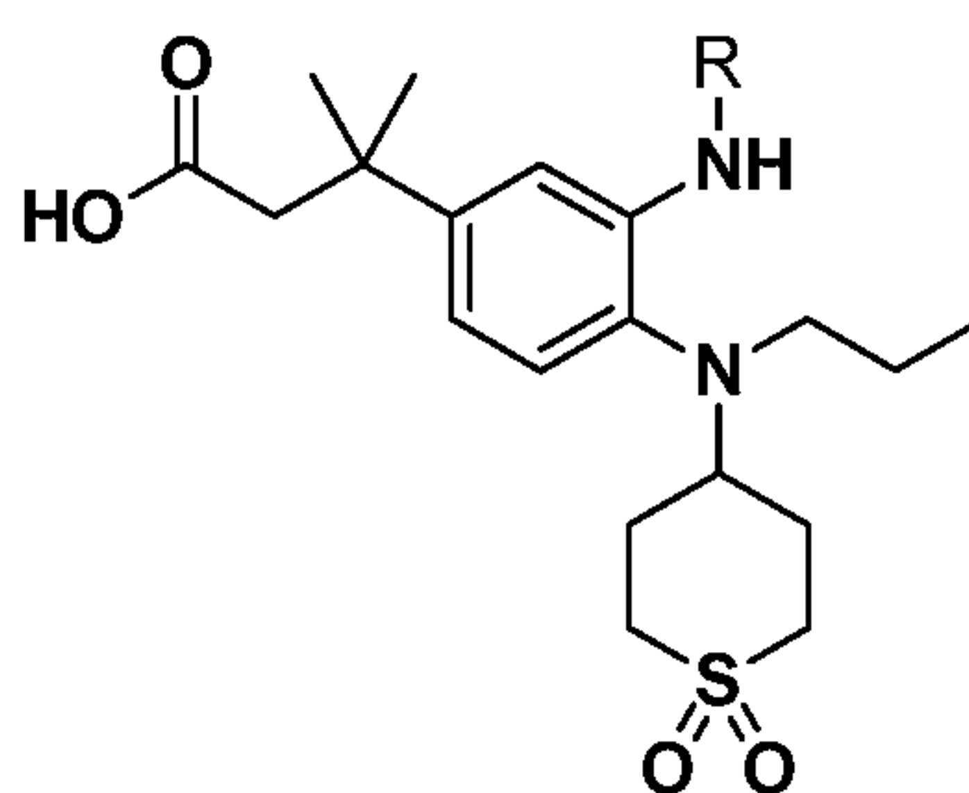
Examples 188 and 189
