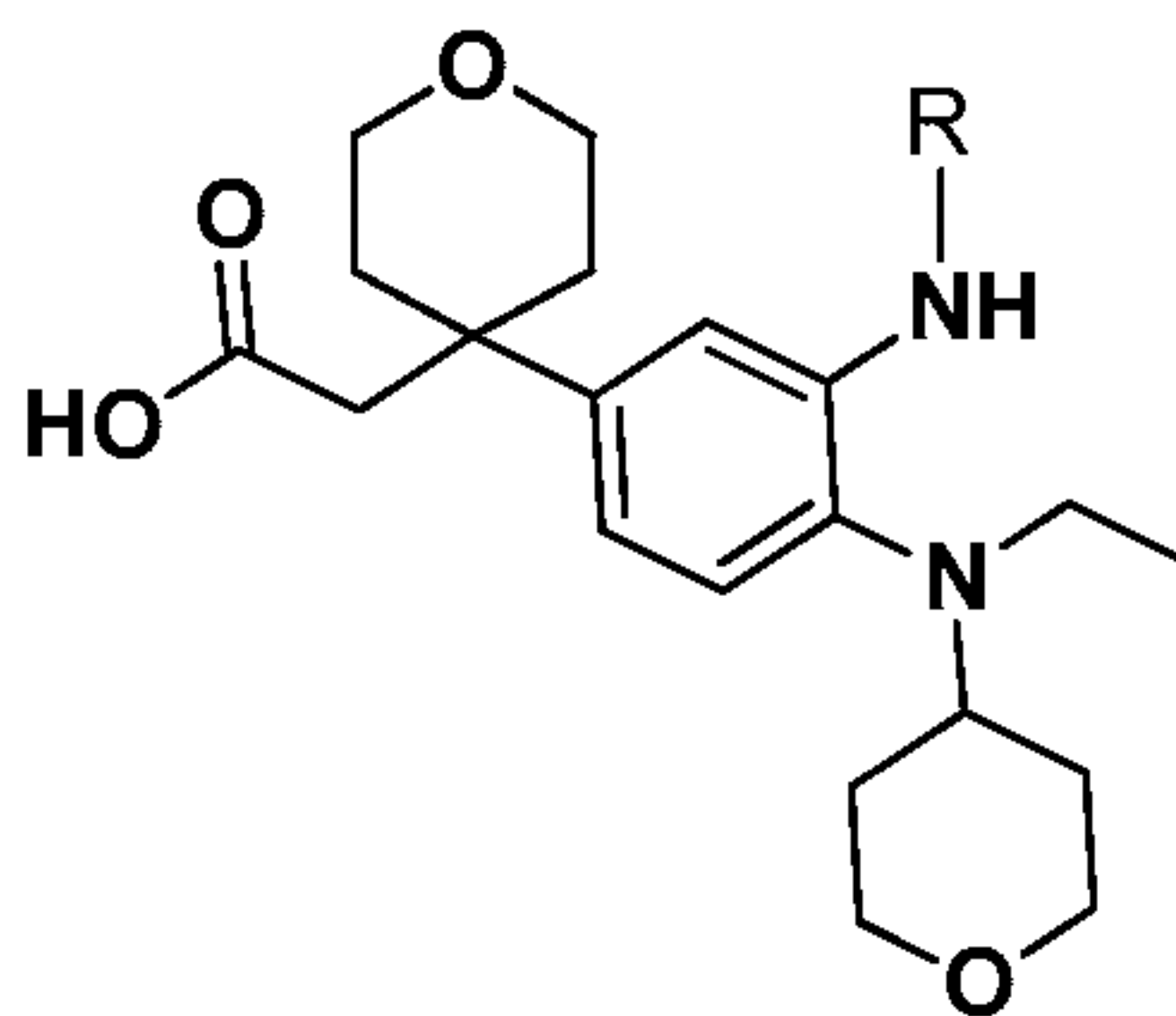
Examples 154 to 156
