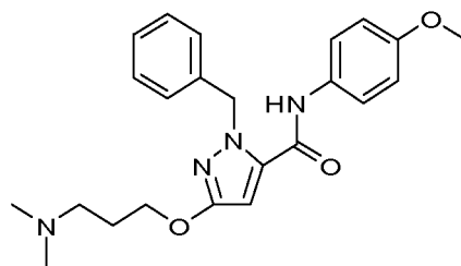
CFM-1571 (see patent publication WO2000027394)
