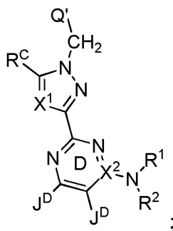
Formula III' a
