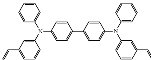
Positive hole transport material 1
