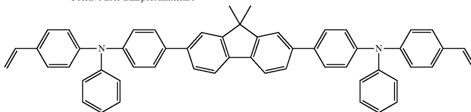
Positive hole transport material 6
