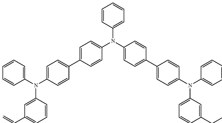
Positive hole transport material 4
