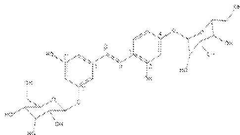
Mulberroside A
