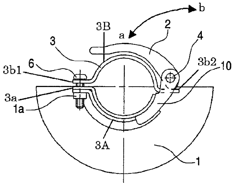
Fig. 9 Related Art
