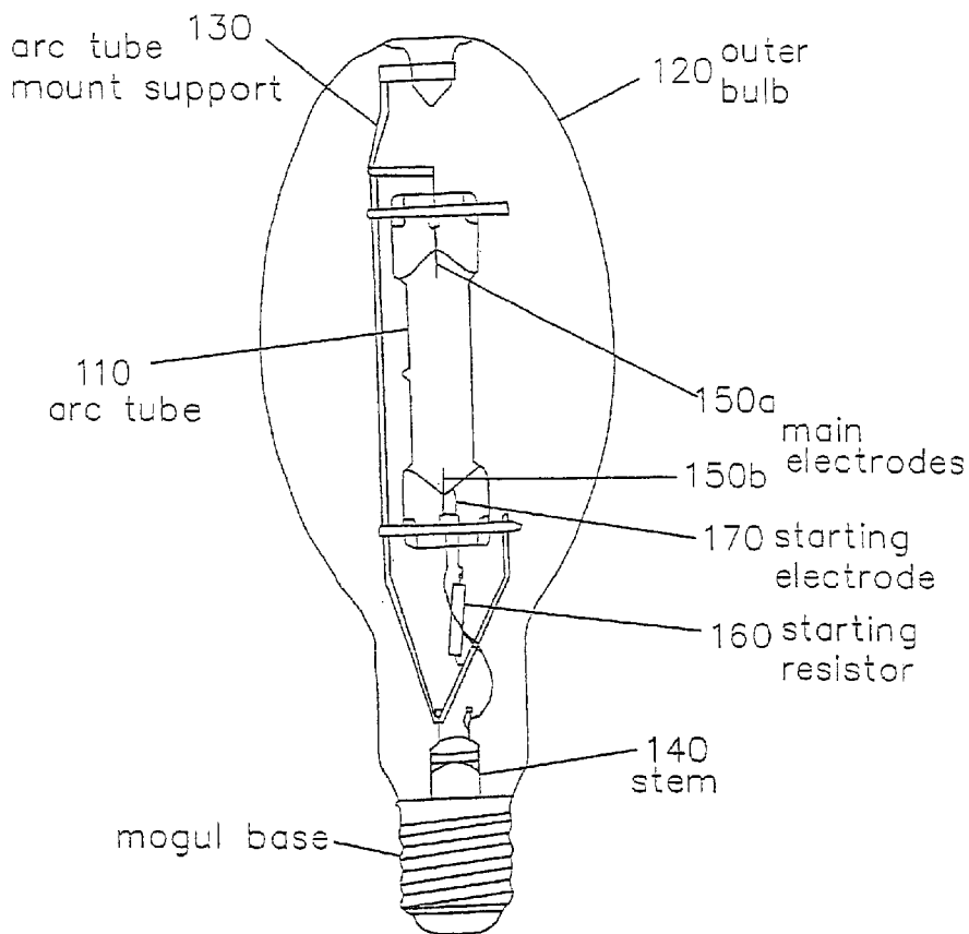
High-pressure mercury-vapor lamp
