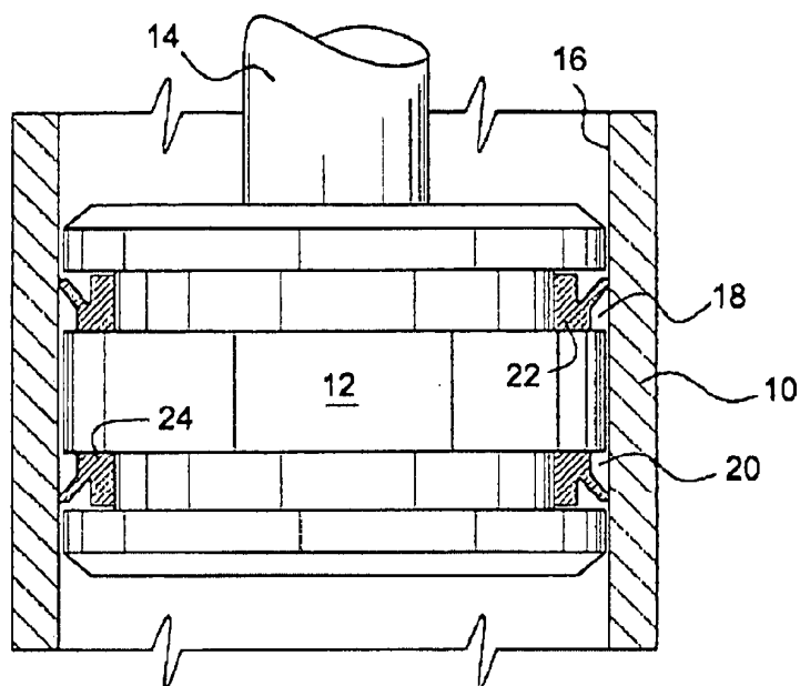
FIG. 1 (PRIOR ART)
