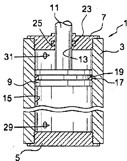
FIG. 2 (PRIOR ART)
