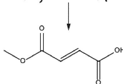
Monomethyl fumarate ( MMF )
