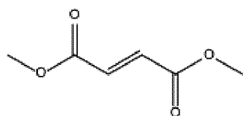
Dimethyl fumarate ( DMF )
