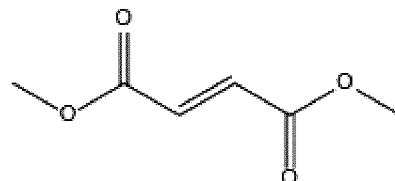
Dimethyl fumarate ( DMF )
