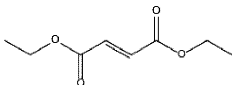
Diethyl fumarate ( DEF )
