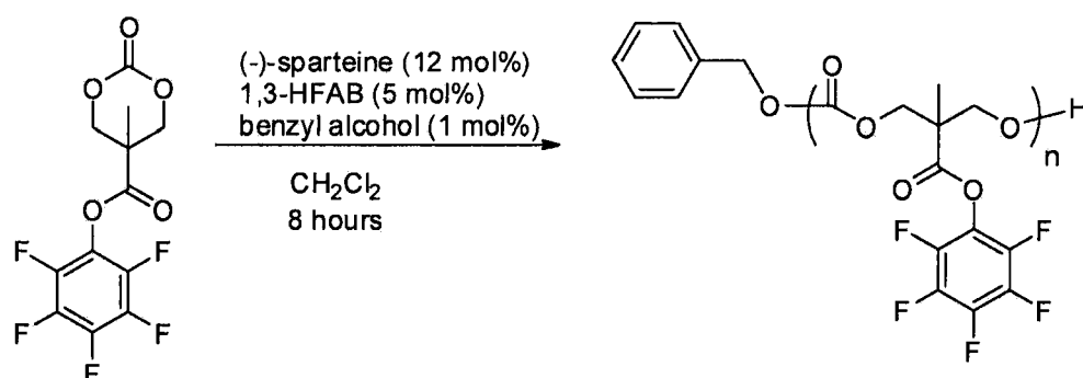
MTC-PhF 5
