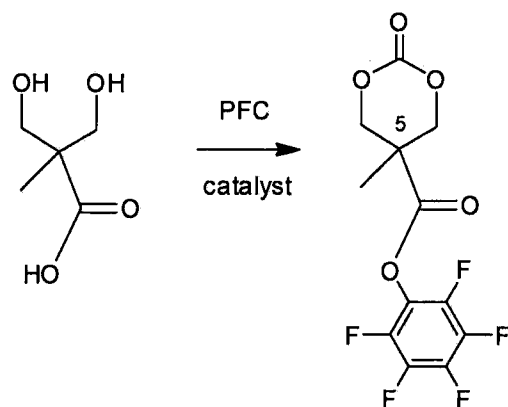
Bis-MPA, (8)
