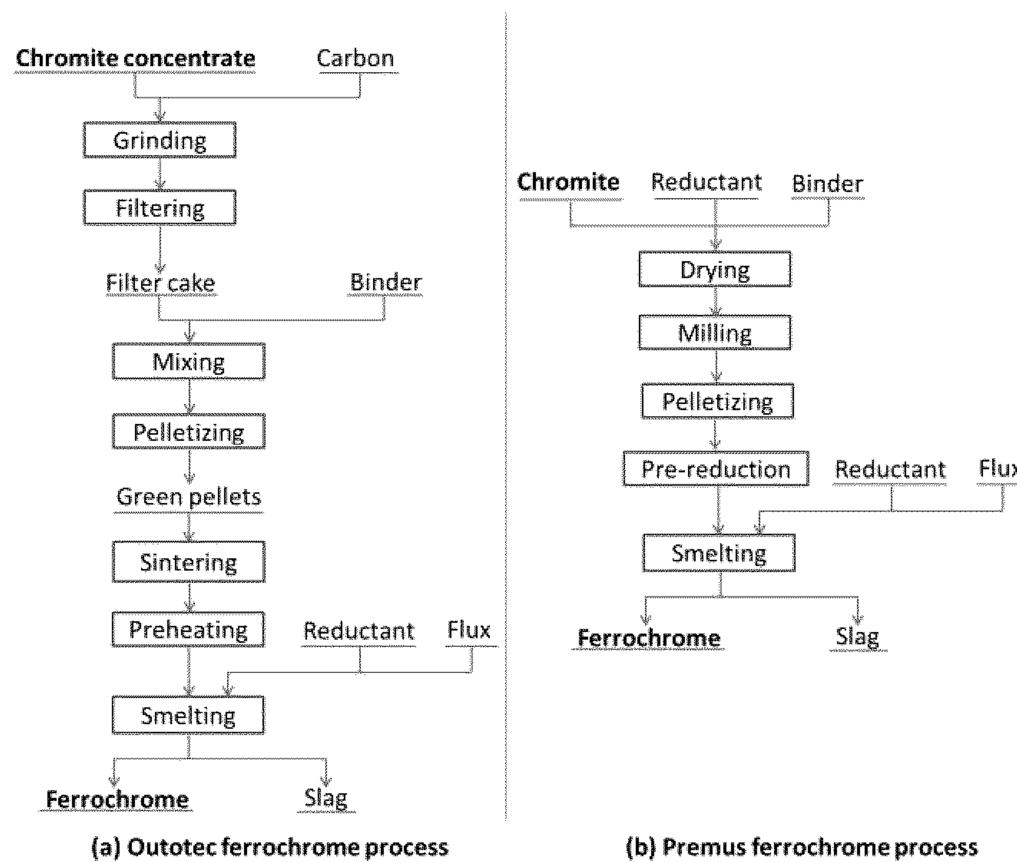
Figure 1 (PRIOR ART)
