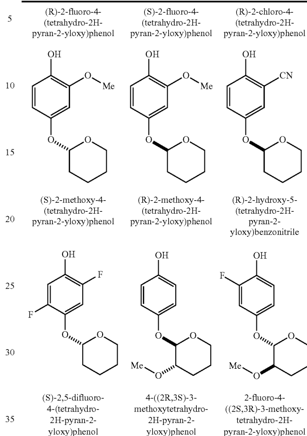
Examples: Cyclic deoxyArbutins
