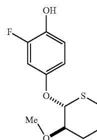
2-fluoro-4-((2R,3R)-3-methoxytetrahydro-2H-thiopyran-2-yloxy)phenol
