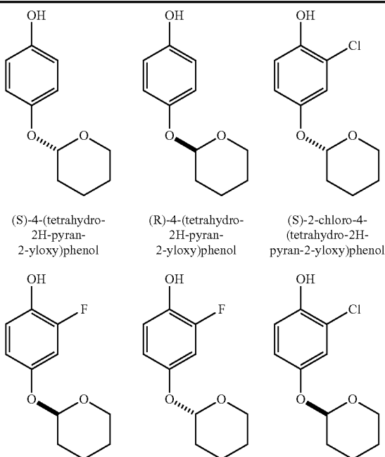
Examples: Cyclic deoxyArbutins
