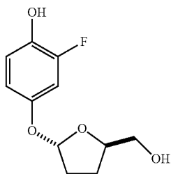
2-fluoro-4-((2S,5R)-5- (hydroxymethyl)- tetrahydrofuran- 2-yloxy)phenol
