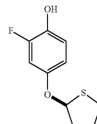
(S)-2-fluoro-4-(tetrahydrothiophen-2-yloxy)phenol
