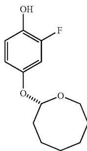
(S)-2-fluoro-4-(oxocan-2-yloxy)phenol
