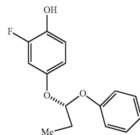
(S)-2-fluoro-4-(1-phenoxypropoxy)phenol
