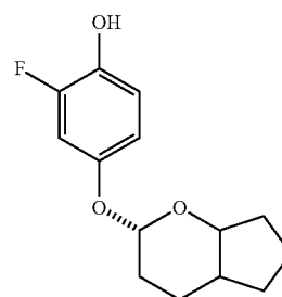
2-fluoro-4-((2S)- octahydrocyclopenta[b]pyran-2- yloxy)phenol
