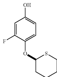
(R)-3-fluoro-4-(tetrahydro-2H-thiopyran-2-yloxy)phenol
