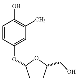
4-((2S,5S)-5- (hydroxymethyl)- tetrahydrofuran-2- yloxy)-2-methylphenol
