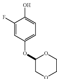
(R)-4-(1,4-dioxan-2-yloxy)-2-fluorophenol
