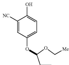
(R)-5-(1-ethoxypropoxy)-2-hydroxybenzonitrile
