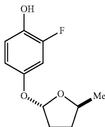
2-fluoro-4-((2S,5S)-5- methyltetrahydrofuran-2- yloxy)phenol
