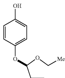
(R)-4-(1-ethoxypropoxy)phenol
