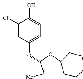
(S)-2-chloro-4-(1-(cyclohexyloxy)propoxy)phenol
