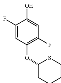
(R)-2,5-difluoro-4-(tetrahydro-2H-thiopyran-2-yloxy)phenol
