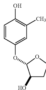
(2S,3R)-2-(4-hydroxy-3- methylphenoxy)- tetrahydrofuran-3-ol
