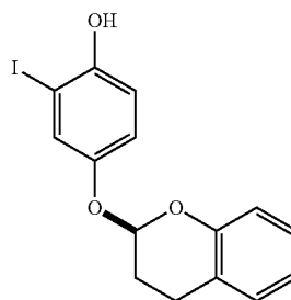
(S)-4-(chroman-2-yloxy)-2-iodophenol
