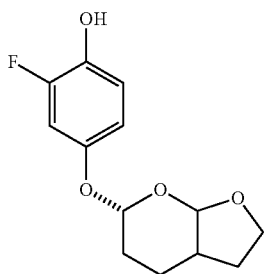
2-fluoro-4-((6R)-hexahydro-2H-furo[2,3-b]pyran-6-yloxy)phenol
