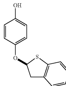
(S)-4-(2,3-dihydrobenzo[b]thiophen-2-yloxy)phenol
