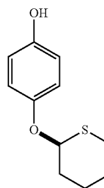
(S)-4-(tetrahydro-2H-thiopyran-2-yloxy)phenol
