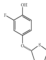
(R)-2-fluoro-4-(tetrahydrothiophen-2-yloxy)phenol
