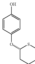
(R)-4-(tetrahydro-2H-thiopyran-2-yloxy)phenol
