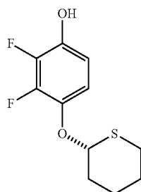
(S)-3-fluoro-4-(tetrahydro-2H-thiopyran-2-yloxy)phenol
