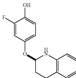
(R)-2-fluoro-4-(1,2,3,4-tetrahydroquinolin-2-yloxy)phenol
