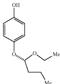
(R)-4-(1-ethoxypropoxy)phenol
