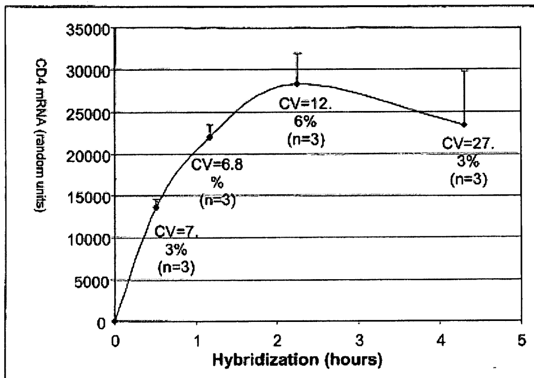
FIG 9. Hybridization kinetics
