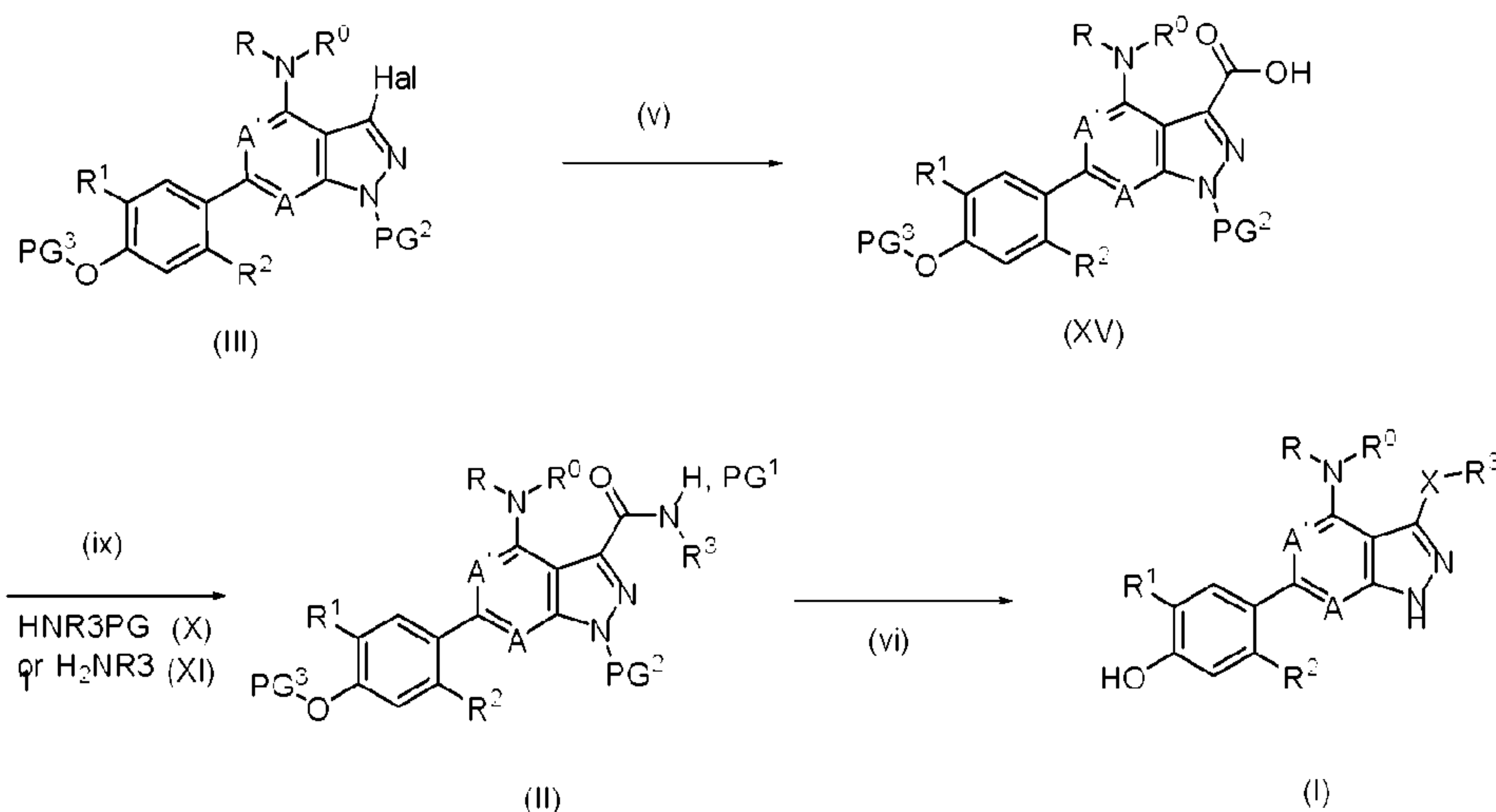
Scheme 3
