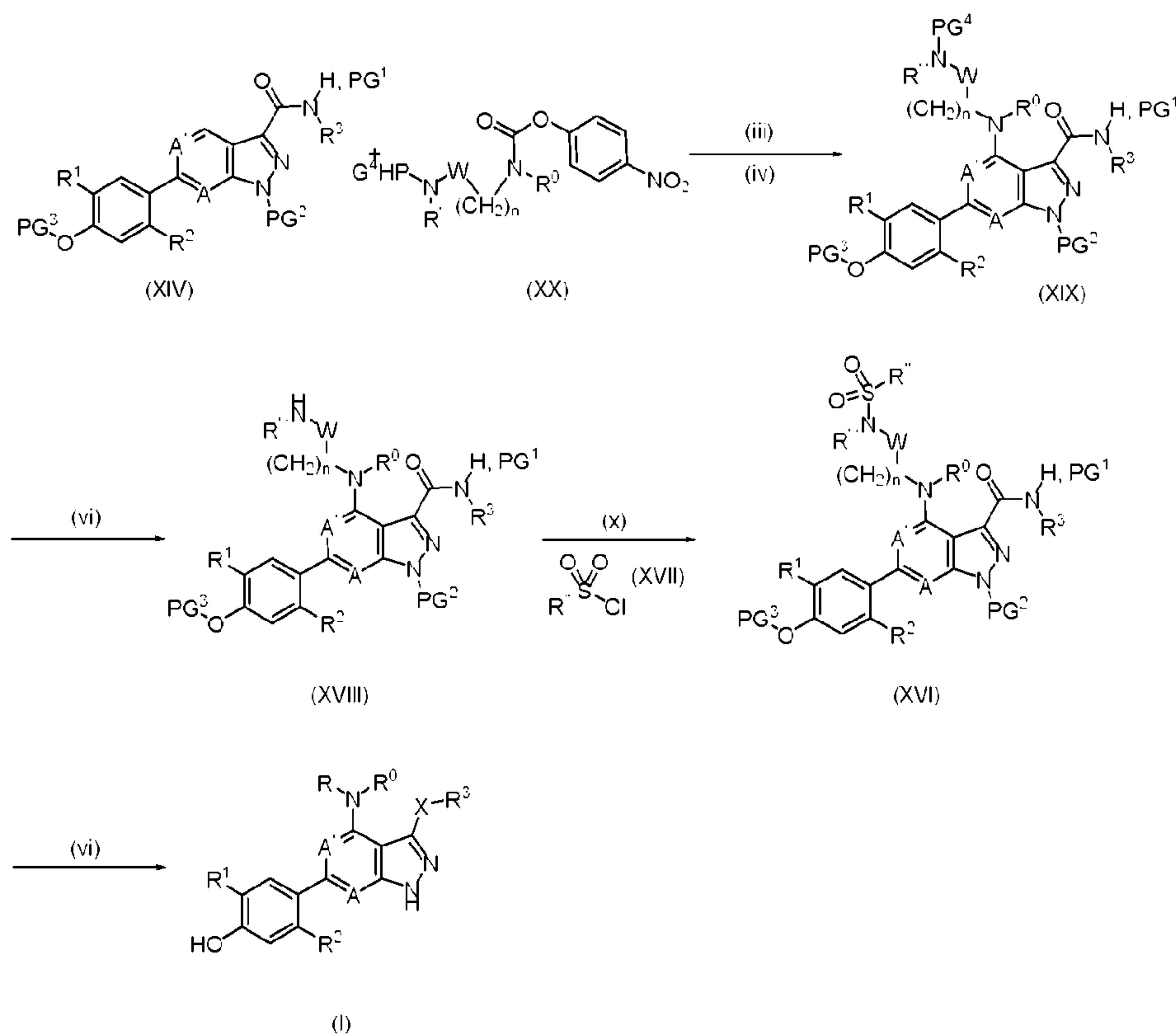
Scheme 4
