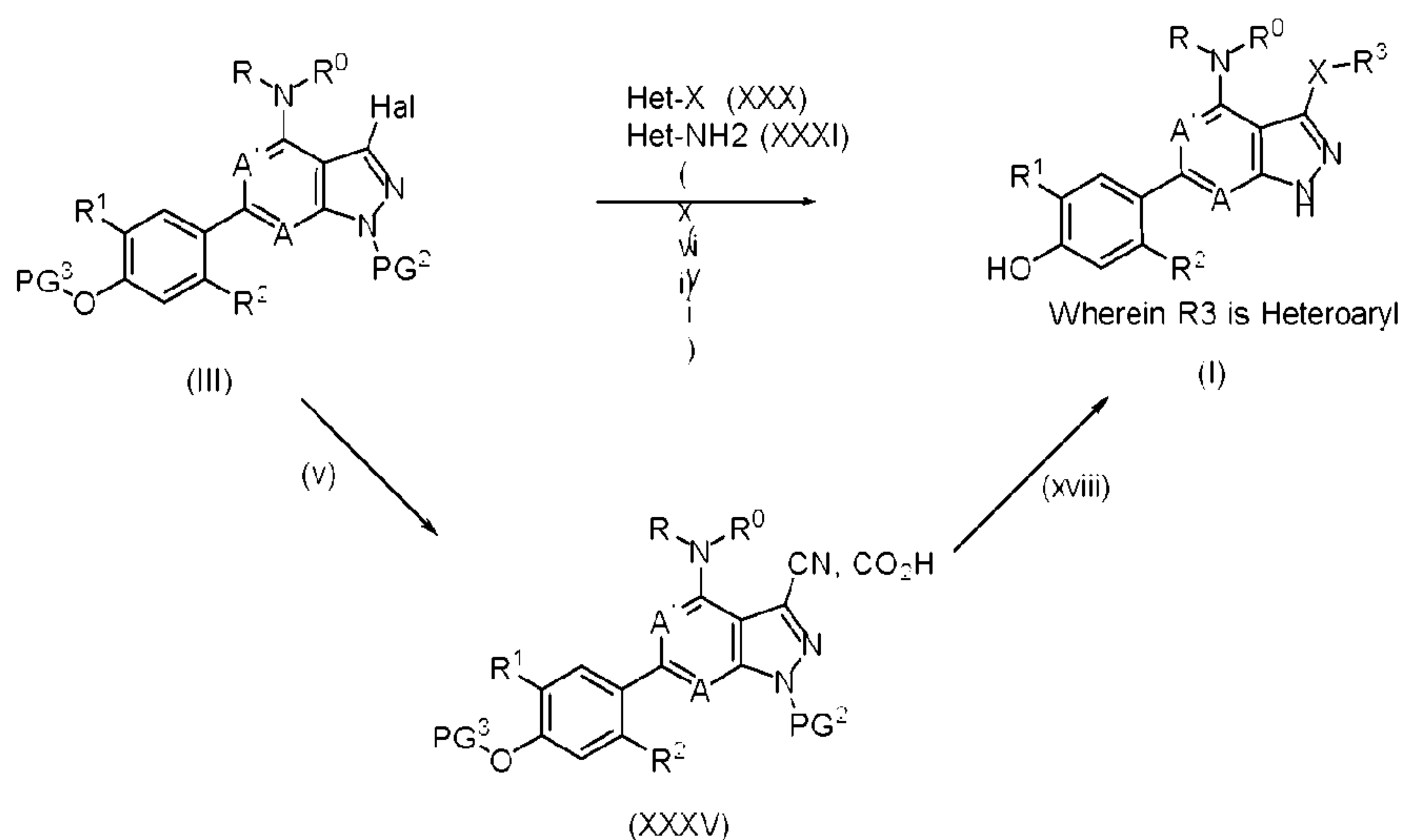
Scheme 7
