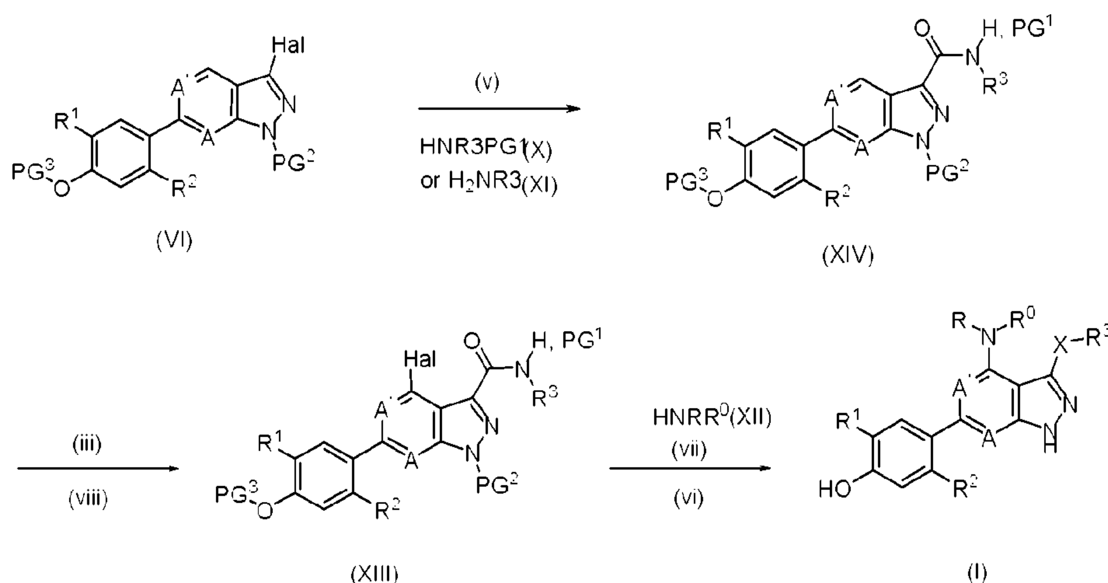
Scheme 2
