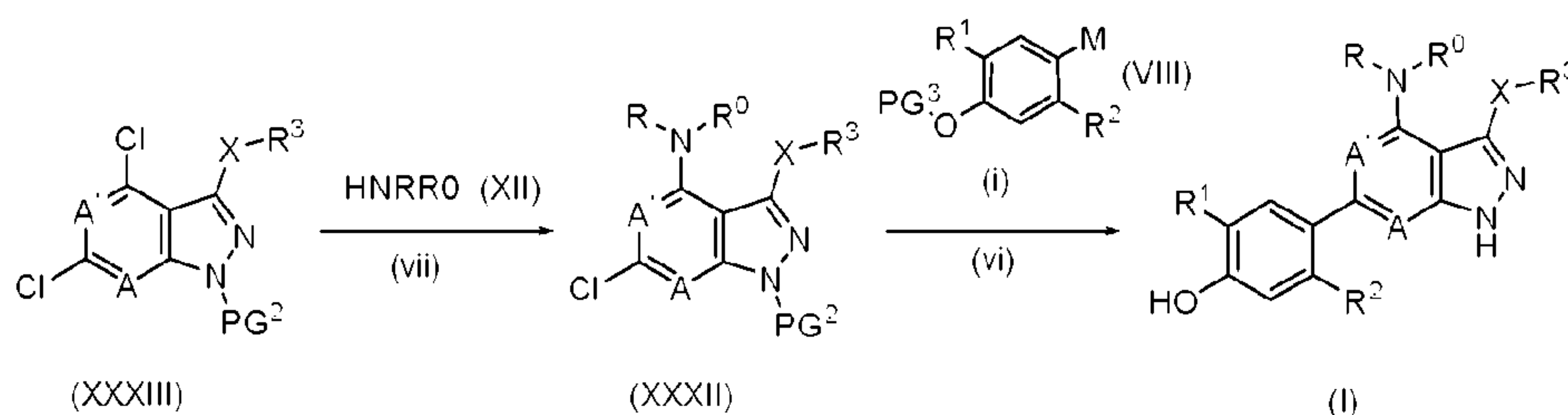
Scheme 8
