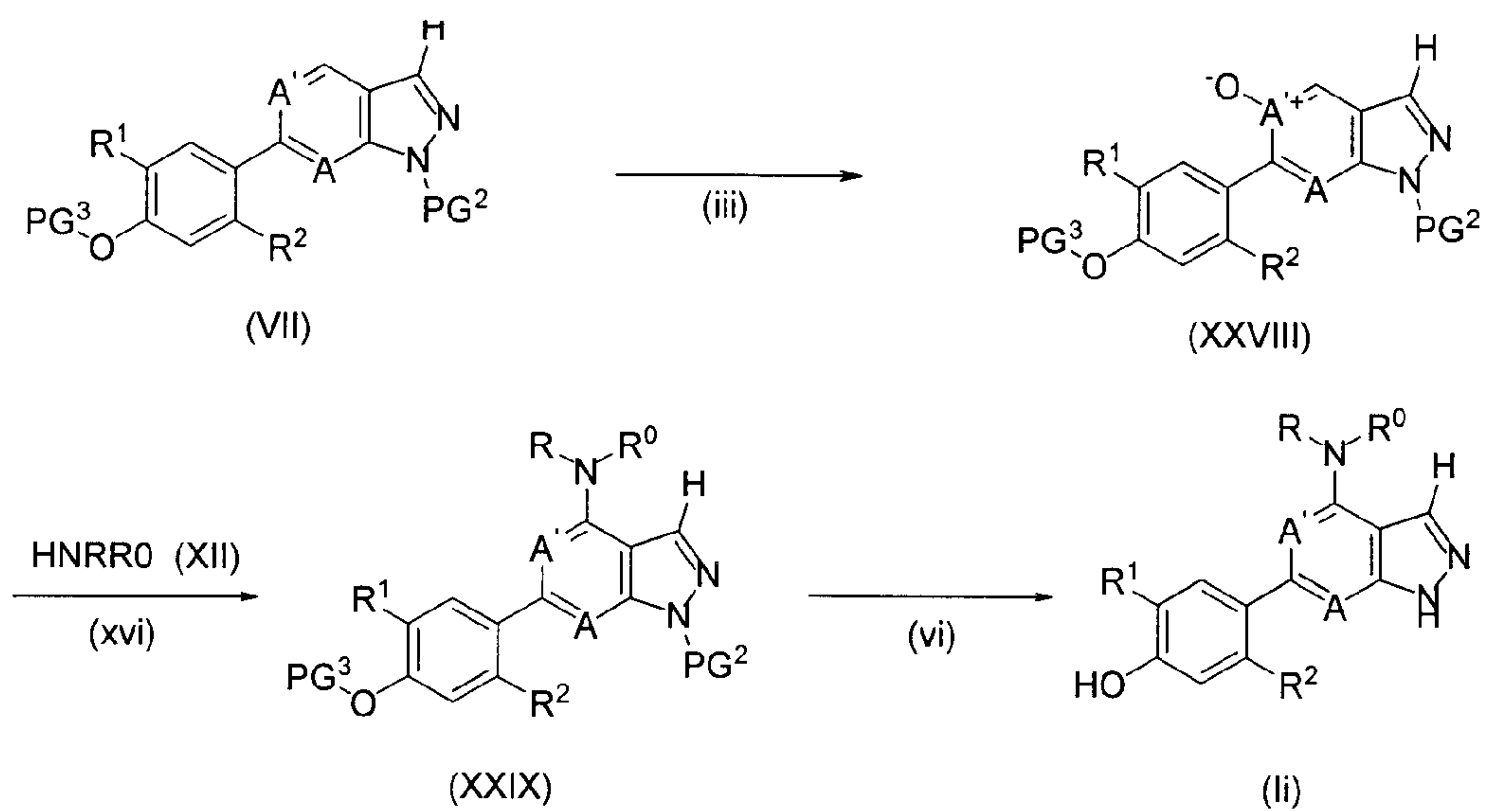
Scheme 6
