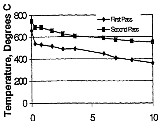
Temperature Profiles For Gas/Solids Contacting - Example 2
