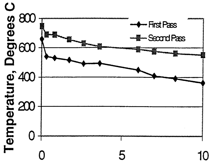
Figure 1: Temperature Profiles For Gas/Solids Contacting - Example 2
