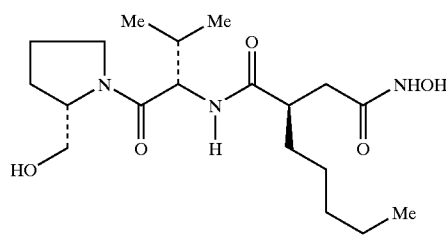
Actinonin
